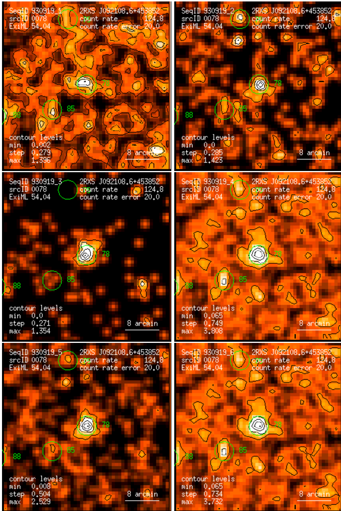
Figure 78: RASS 930919: detection 0078: band rate images, Gaussian filter: (1) PSPC channels 11 – 41, (2) 52 – 90, (3) 91 – 201, (4) 11 – 235, (5) 52 – 201, (6) 11 – 201. Broad band rates in counts/ks. Band rate contour levels in counts/ks/arcmin 2 .
