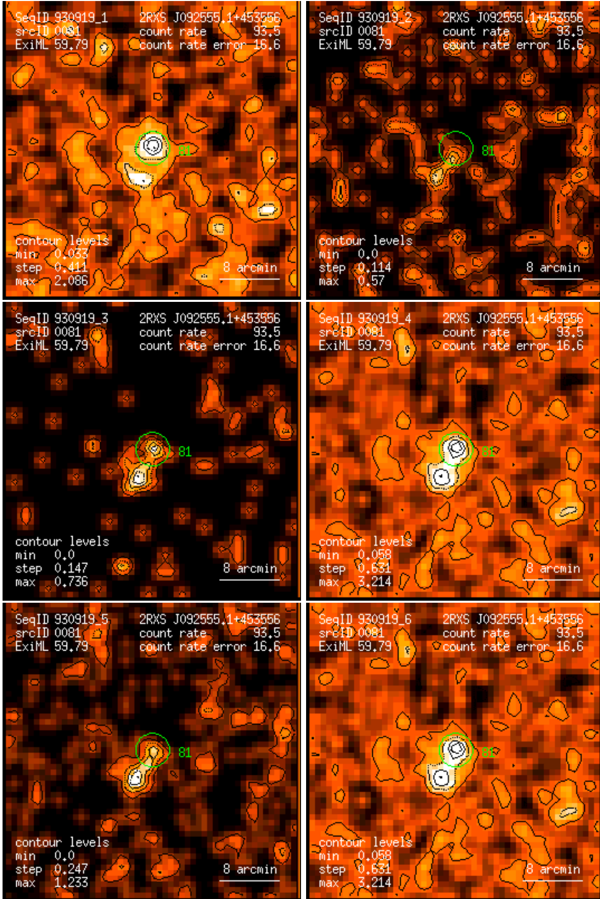
Figure 81: RASS 930919: detection 0081: band rate images, Gaussian filter: (1) PSPC channels 11 – 41, (2) 52 – 90, (3) 91 – 201, (4) 11 – 235, (5) 52 – 201, (6) 11 – 201. Broad band rates in counts/ks. Band rate contour levels in counts/ks/arcmin 2 .
