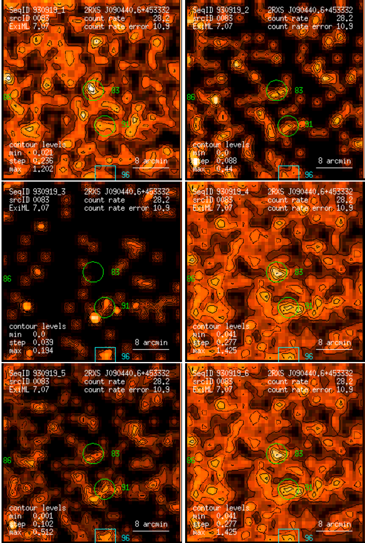
Figure 83: RASS 930919: detection 0083: band rate images, Gaussian filter: (1) PSPC channels 11 – 41, (2) 52 – 90, (3) 91 – 201, (4) 11 – 235, (5) 52 – 201, (6) 11 – 201. Broad band rates in counts/ks. Band rate contour levels in counts/ks/arcmin 2 .
