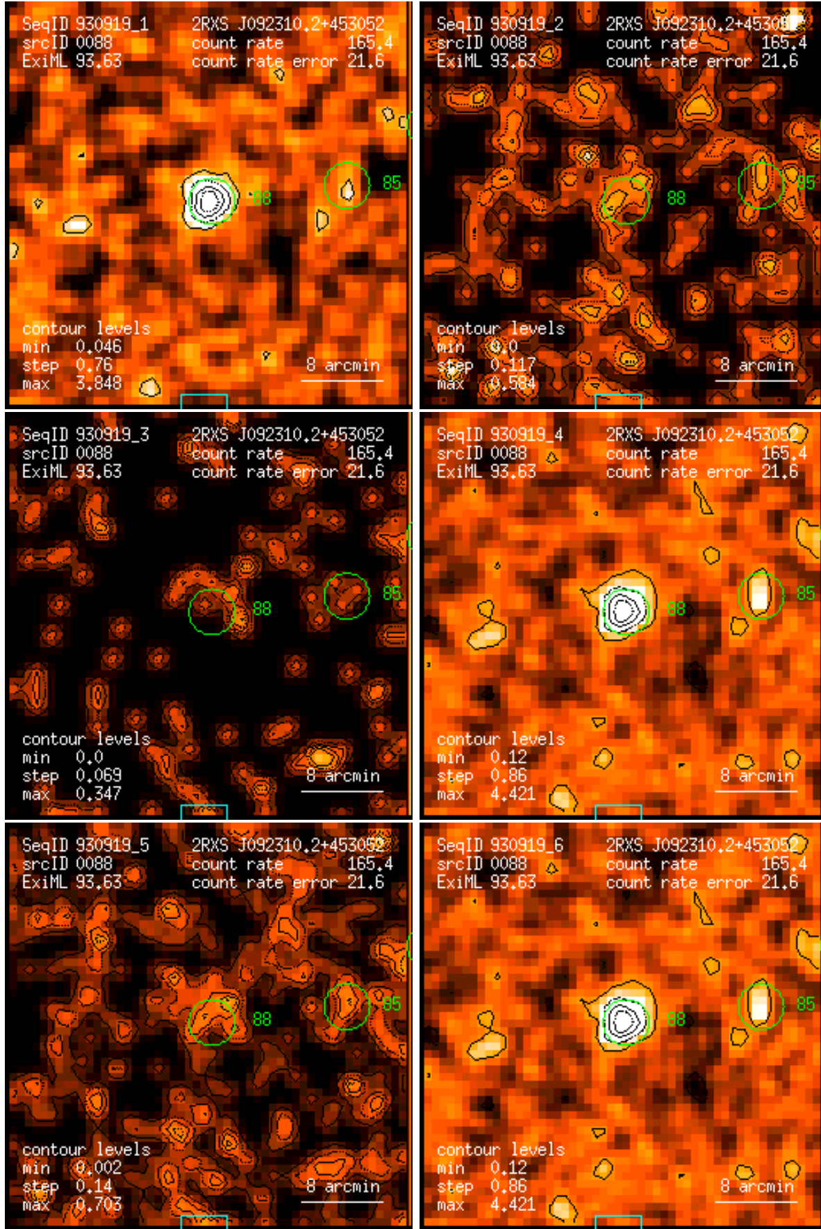
Figure 88: RASS 930919: detection 0088: band rate images, Gaussian filter: (1) PSPC channels 11 – 41, (2) 52 – 90, (3) 91 – 201, (4) 11 – 235, (5) 52 – 201, (6) 11 – 201. Broad band rates in counts/ks. Band rate contour levels in counts/ks/arcmin 2 .
