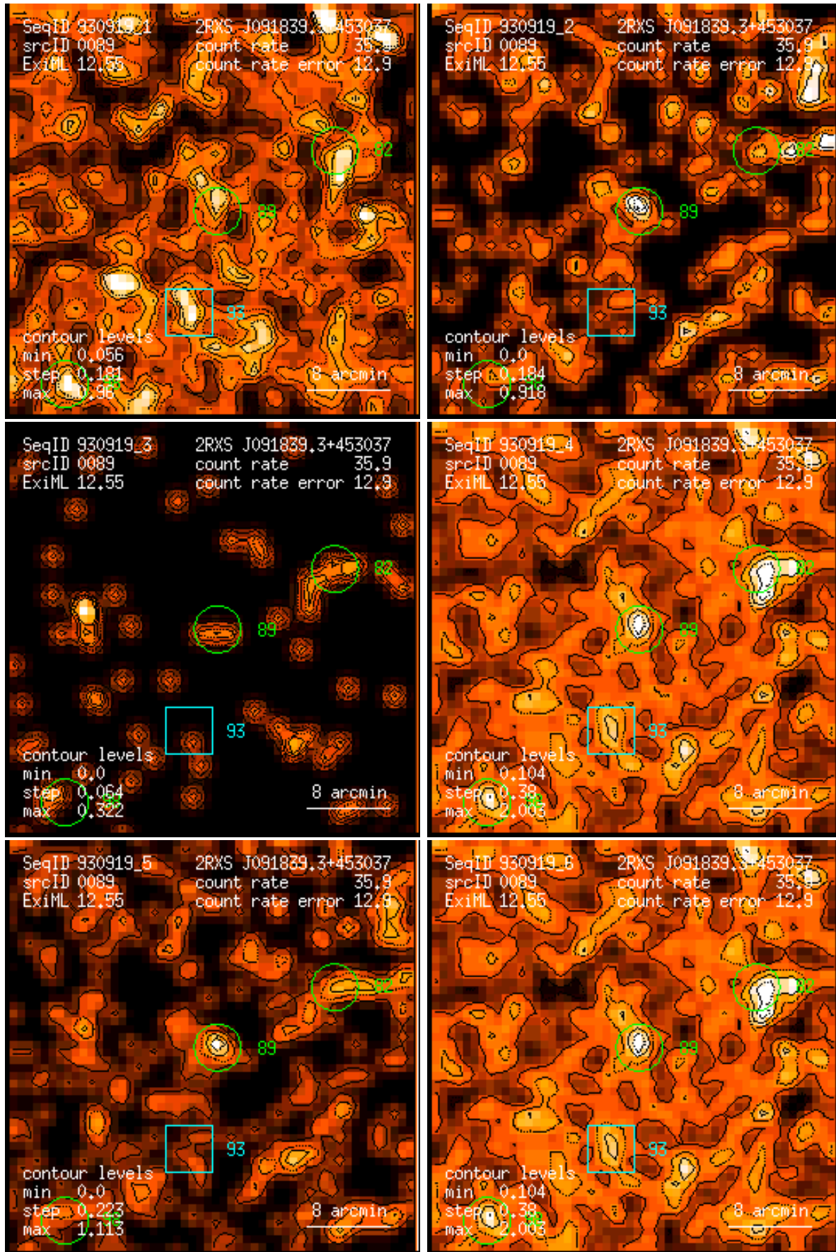
Figure 89: RASS 930919: detection 0089: band rate images, Gaussian filter: (1) PSPC channels 11 – 41, (2) 52 – 90, (3) 91 – 201, (4) 11 – 235, (5) 52 – 201, (6) 11 – 201. Broad band rates in counts/ks. Band rate contour levels in counts/ks/arcmin 2 .
