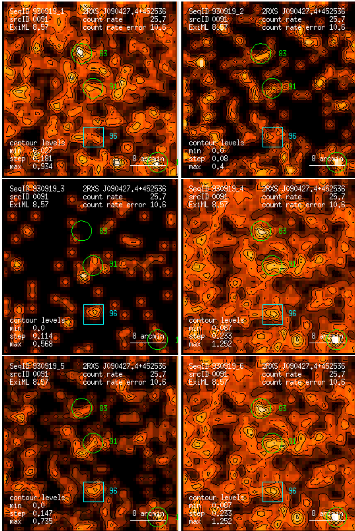
Figure 91: RASS 930919: detection 0091: band rate images, Gaussian filter: (1) PSPC channels 11 – 41, (2) 52 – 90, (3) 91 – 201, (4) 11 – 235, (5) 52 – 201, (6) 11 – 201. Broad band rates in counts/ks. Band rate contour levels in counts/ks/arcmin 2 .
