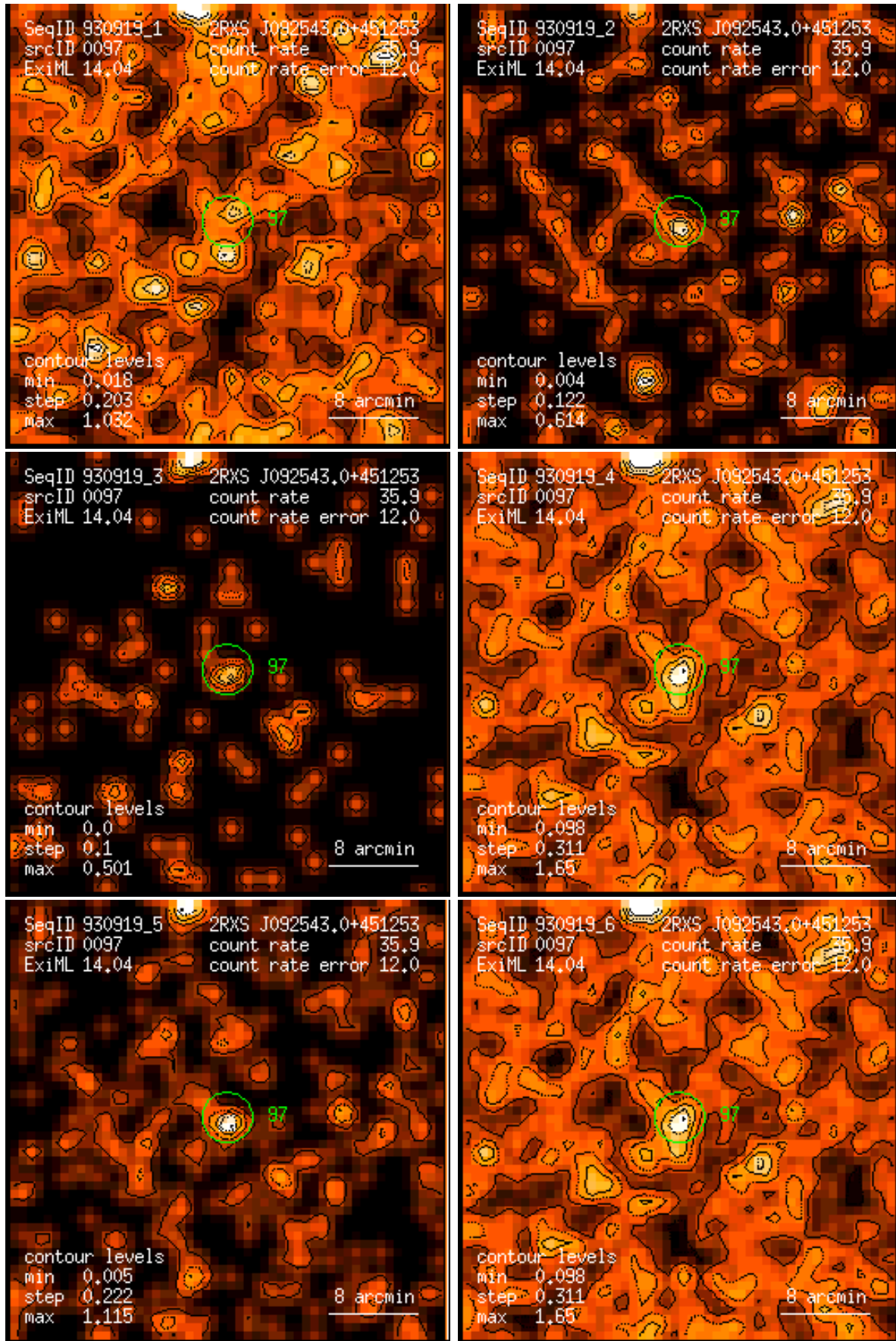
Figure 97: RASS 930919: detection 0097: band rate images, Gaussian filter: (1) PSPC channels 11 – 41, (2) 52 – 90, (3) 91 – 201, (4) 11 – 235, (5) 52 – 201, (6) 11 – 201. Broad band rates in counts/ks. Band rate contour levels in counts/ks/arcmin 2 .
