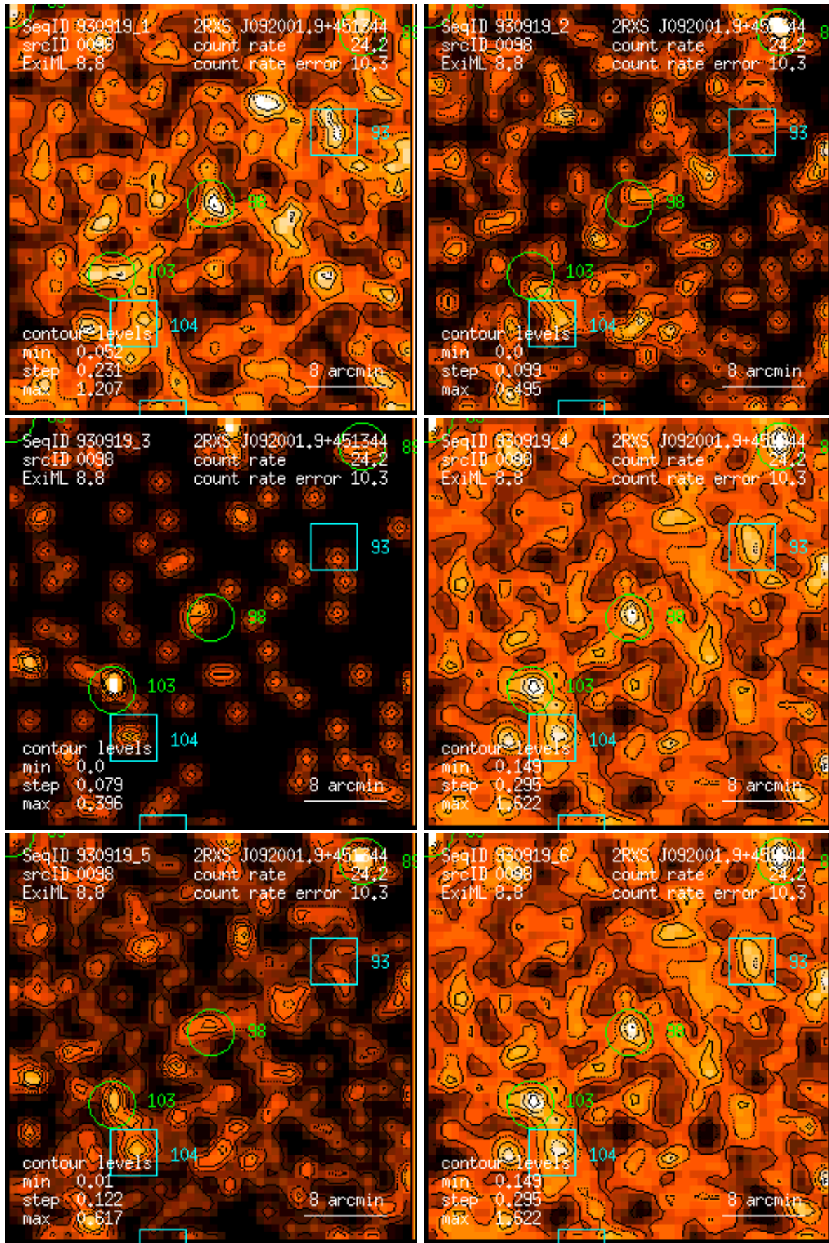
Figure 98: RASS 930919: detection 0098: band rate images, Gaussian filter: (1) PSPC channels 11 – 41, (2) 52 – 90, (3) 91 – 201, (4) 11 – 235, (5) 52 – 201, (6) 11 – 201. Broad band rates in counts/ks. Band rate contour levels in counts/ks/arcmin 2 .
