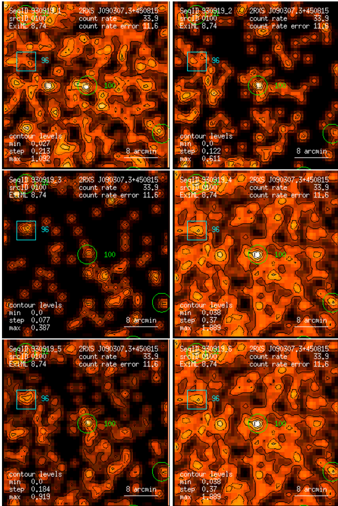
Figure 100: RASS 930919: detection 0100: band rate images, Gaussian filter: (1) PSPC channels 11 – 41, (2) 52 – 90, (3) 91 – 201, (4) 11 – 235, (5) 52 – 201, (6) 11 – 201. Broad band rates in counts/ks. Band rate contour levels in counts/ks/arcmin 2 .
