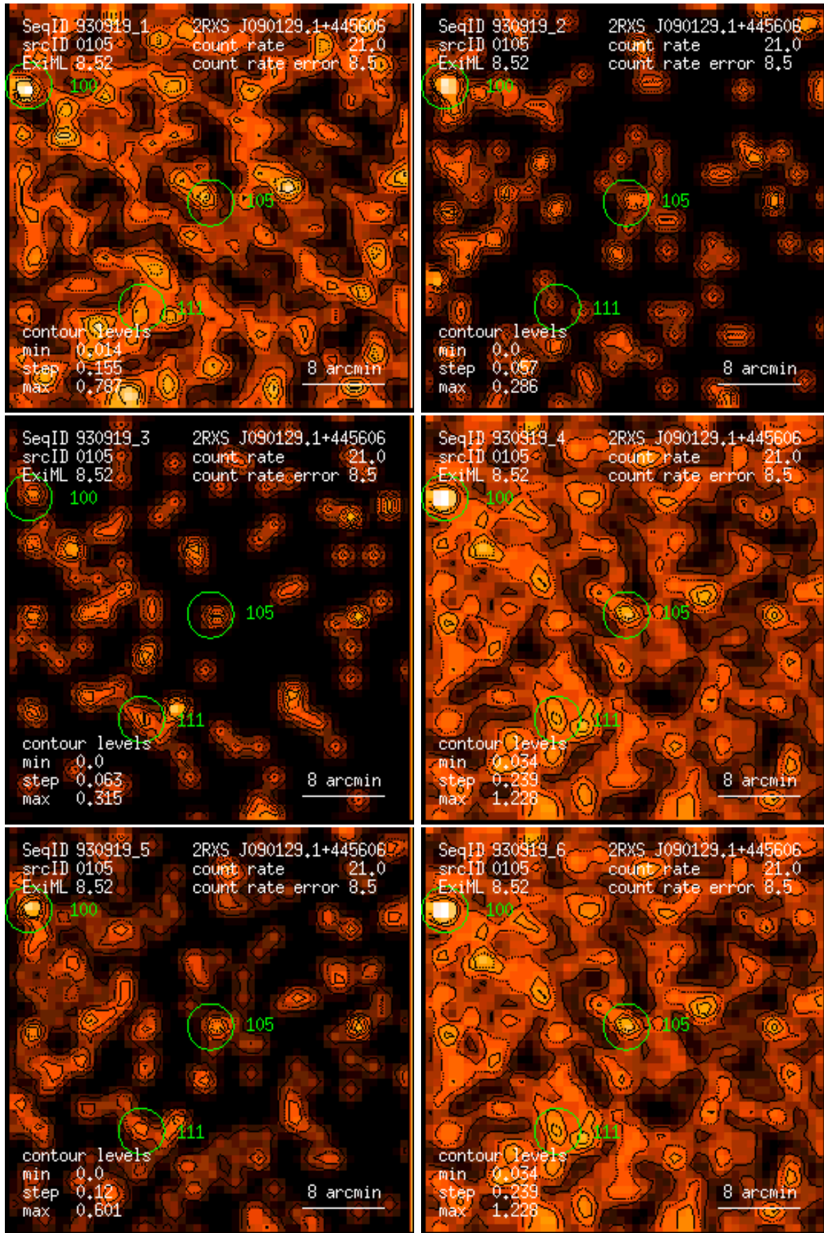
Figure 105: RASS 930919: detection 0105: band rate images, Gaussian filter: (1) PSPC channels 11 – 41, (2) 52 – 90, (3) 91 – 201, (4) 11 – 235, (5) 52 – 201, (6) 11 – 201. Broad band rates in counts/ks. Band rate contour levels in counts/ks/arcmin 2 .
