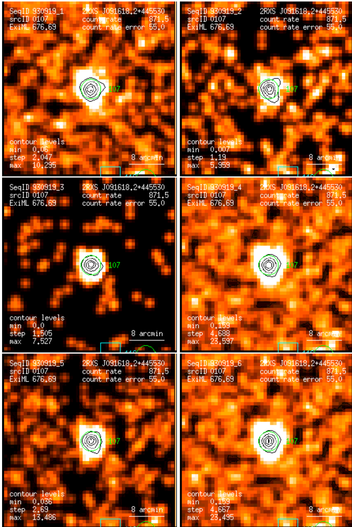
Figure 107: RASS 930919: detection 0107: band rate images, Gaussian filter: (1) PSPC channels 11 – 41, (2) 52 – 90, (3) 91 – 201, (4) 11 – 235, (5) 52 – 201, (6) 11 – 201. Broad band rates in counts/ks. Band rate contour levels in counts/ks/arcmin 2 .
