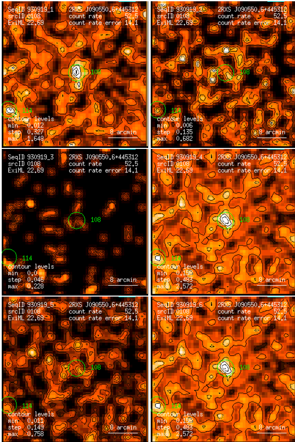
Figure 108: RASS 930919: detection 0108: band rate images, Gaussian filter: (1) PSPC channels 11 – 41, (2) 52 – 90, (3) 91 – 201, (4) 11 – 235, (5) 52 – 201, (6) 11 – 201. Broad band rates in counts/ks. Band rate contour levels in counts/ks/arcmin 2 .
