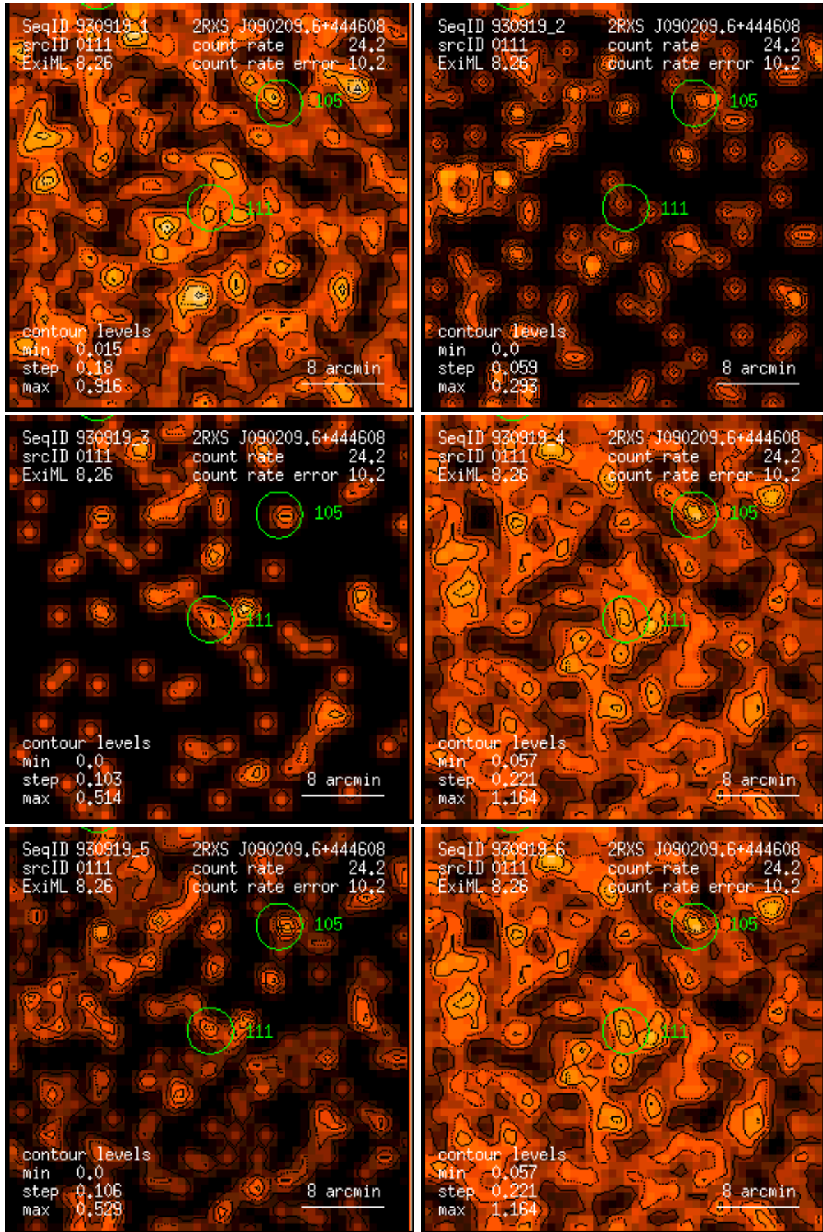
Figure 111: RASS 930919: detection 0111: band rate images, Gaussian filter: (1) PSPC channels 11 – 41, (2) 52 – 90, (3) 91 – 201, (4) 11 – 235, (5) 52 – 201, (6) 11 – 201. Broad band rates in counts/ks. Band rate contour levels in counts/ks/arcmin 2 .
