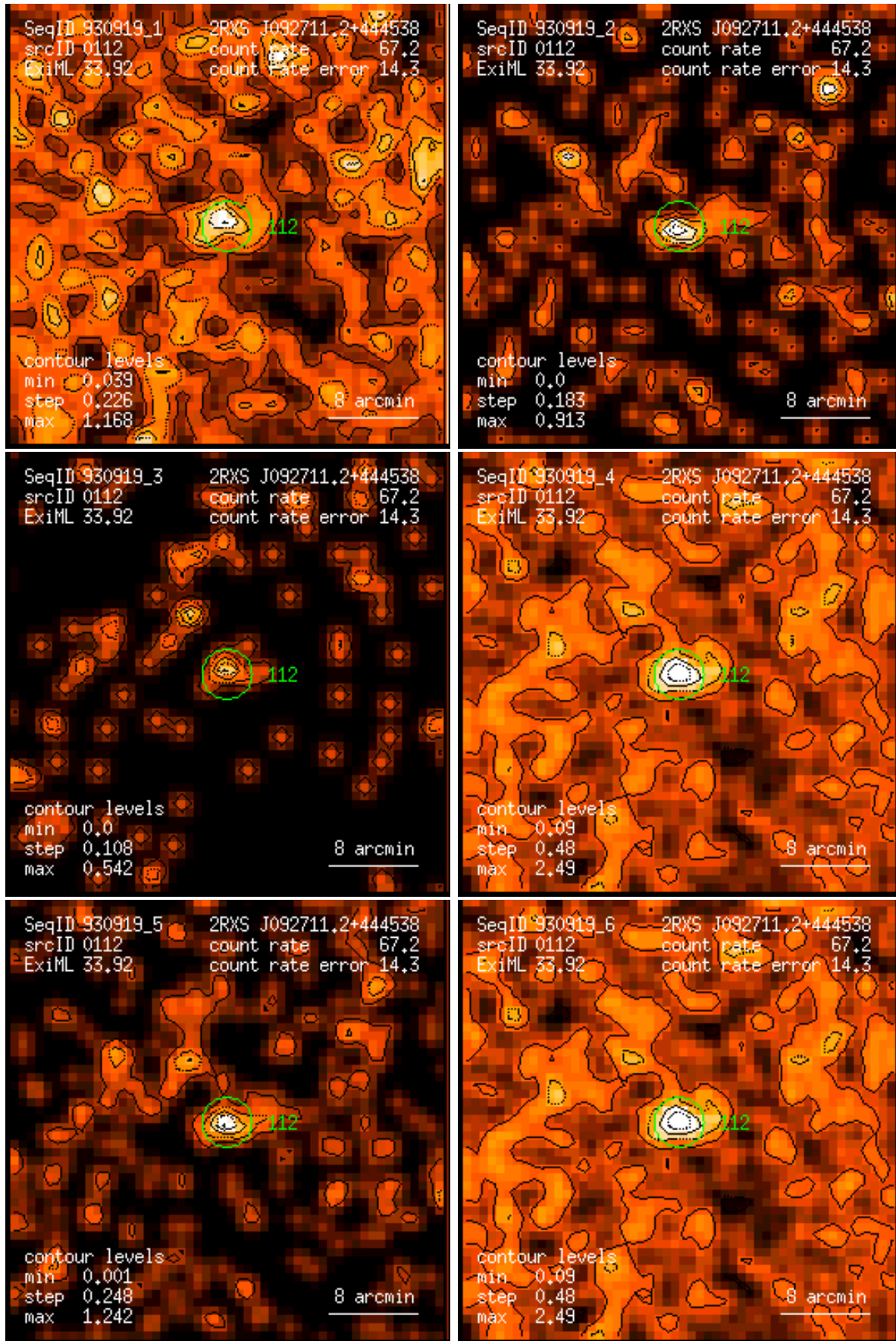
Figure 112: RASS 930919: detection 0112: band rate images, Gaussian filter: (1) PSPC channels 11 – 41, (2) 52 – 90, (3) 91 – 201, (4) 11 – 235, (5) 52 – 201, (6) 11 – 201. Broad band rates in counts/ks. Band rate contour levels in counts/ks/arcmin 2 .
