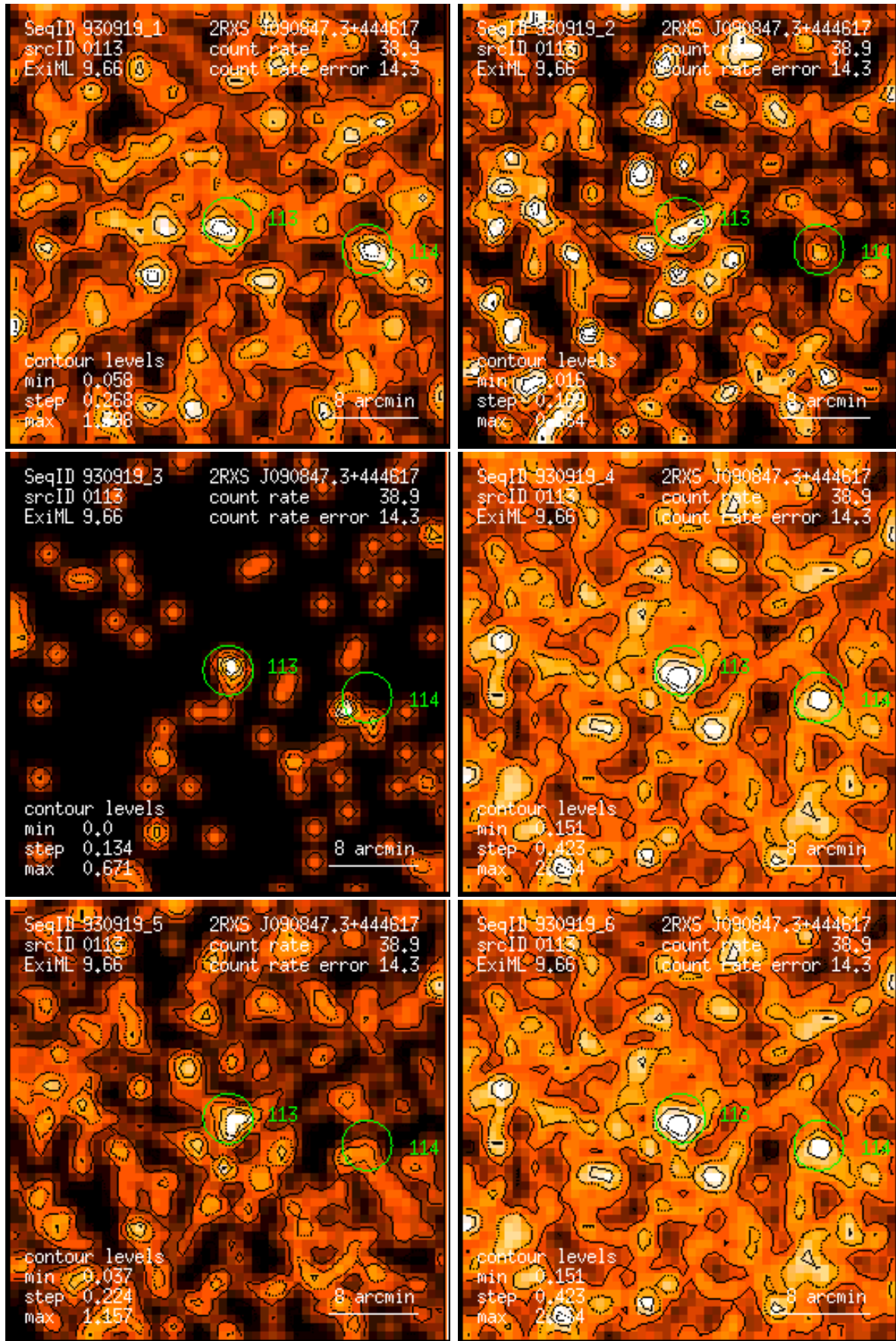
Figure 113: RASS 930919: detection 0113: band rate images, Gaussian filter: (1) PSPC channels 11 – 41, (2) 52 – 90, (3) 91 – 201, (4) 11 – 235, (5) 52 – 201, (6) 11 – 201. Broad band rates in counts/ks. Band rate contour levels in counts/ks/arcmin 2 .
