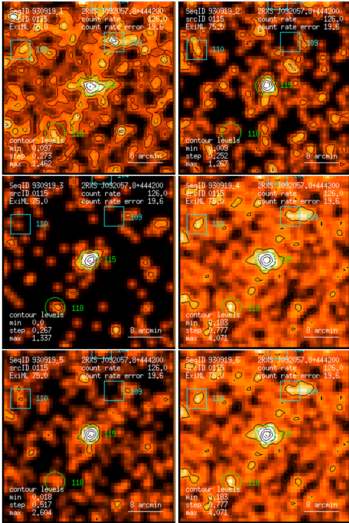
Figure 115: RASS 930919: detection 0115: band rate images, Gaussian filter: (1) PSPC channels 11 – 41, (2) 52 – 90, (3) 91 – 201, (4) 11 – 235, (5) 52 – 201, (6) 11 – 201. Broad band rates in counts/ks. Band rate contour levels in counts/ks/arcmin 2 .
