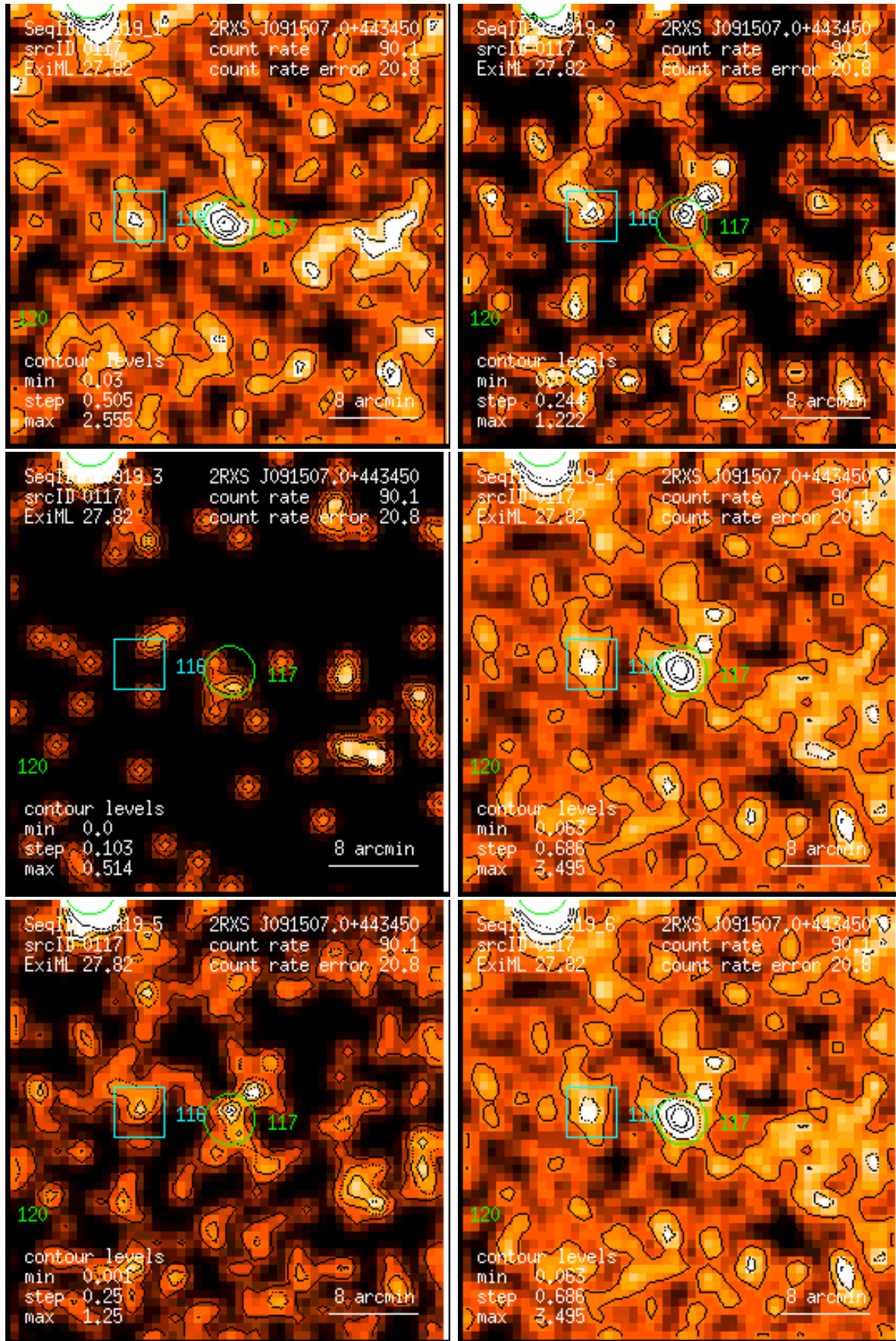
Figure 117: RASS 930919: detection 0117: band rate images, Gaussian filter: (1) PSPC channels 11 – 41, (2) 52 – 90, (3) 91 – 201, (4) 11 – 235, (5) 52 – 201, (6) 11 – 201. Broad band rates in counts/ks. Band rate contour levels in counts/ks/arcmin 2 .
