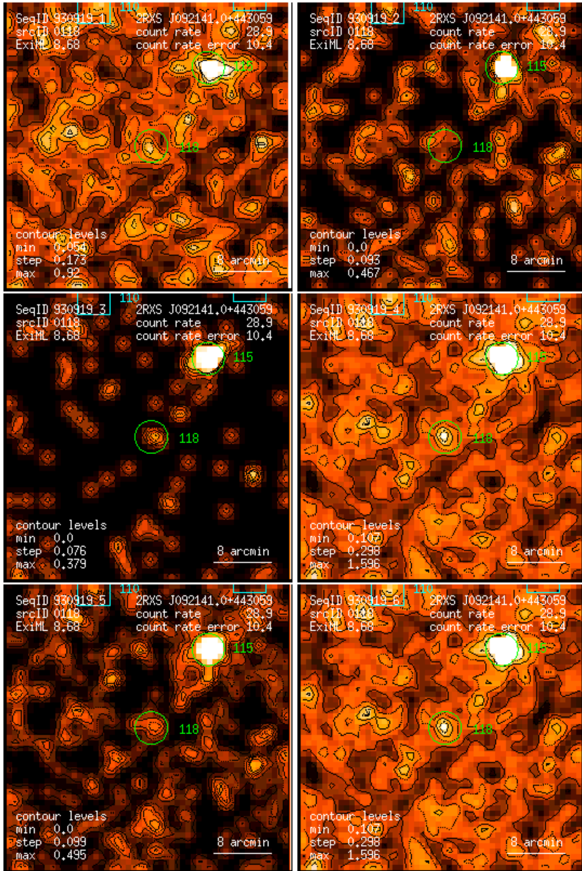
Figure 118: RASS 930919: detection 0118: band rate images, Gaussian filter: (1) PSPC channels 11 – 41, (2) 52 – 90, (3) 91 – 201, (4) 11 – 235, (5) 52 – 201, (6) 11 – 201. Broad band rates in counts/ks. Band rate contour levels in counts/ks/arcmin 2 .
