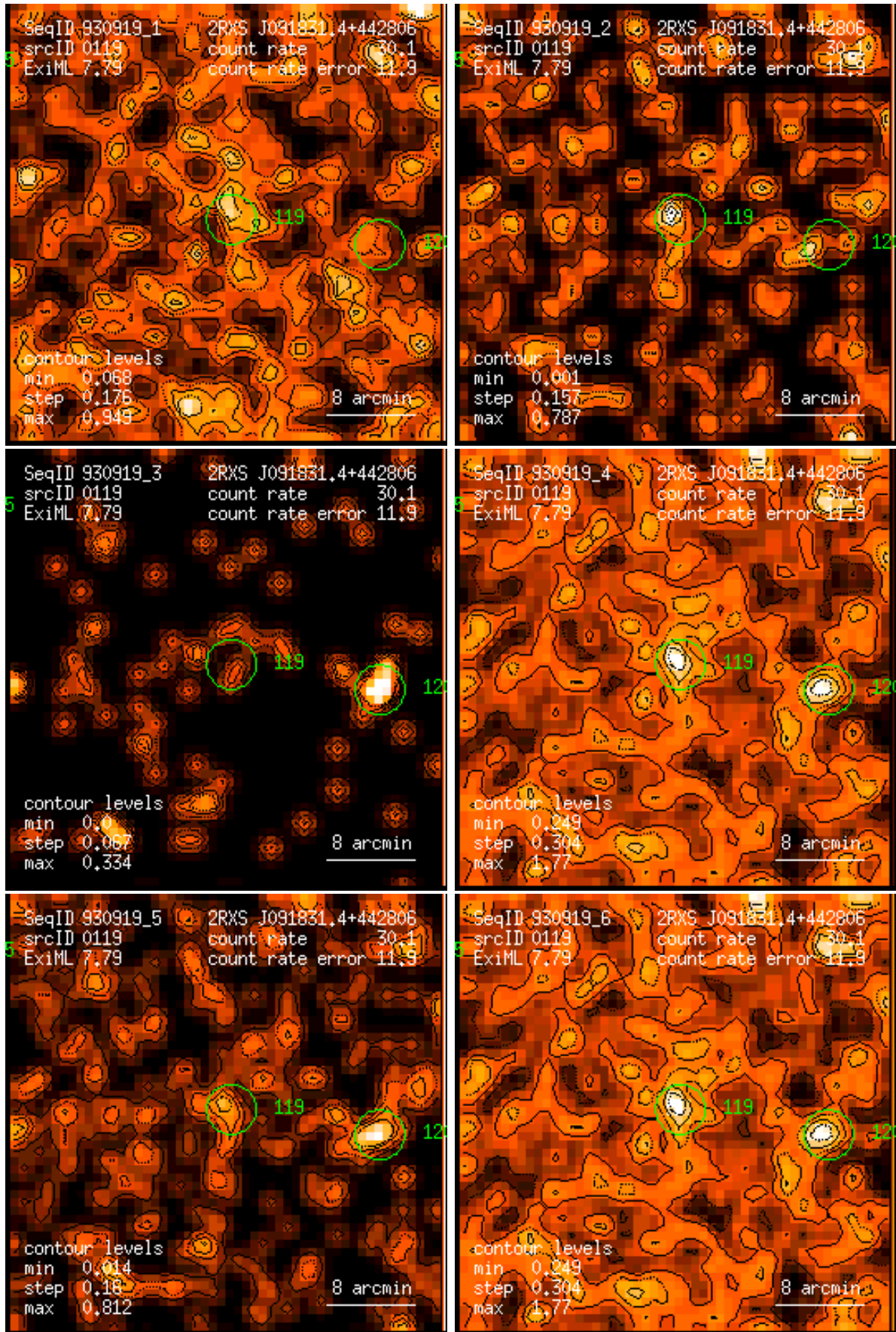
Figure 119: RASS 930919: detection 0119: band rate images, Gaussian filter: (1) PSPC channels 11 – 41, (2) 52 – 90, (3) 91 – 201, (4) 11 – 235, (5) 52 – 201, (6) 11 – 201. Broad band rates in counts/ks. Band rate contour levels in counts/ks/arcmin 2 .
