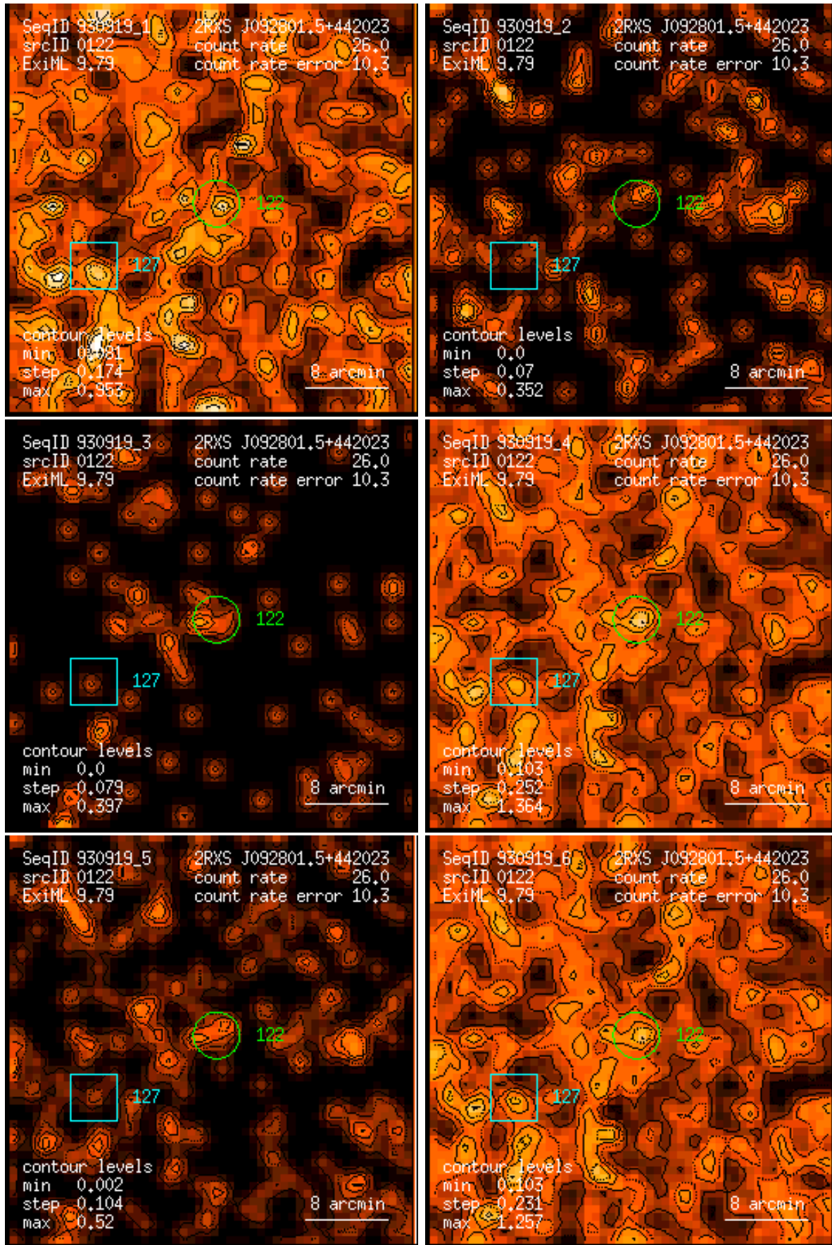
Figure 122: RASS 930919: detection 0122: band rate images, Gaussian filter: (1) PSPC channels 11 – 41, (2) 52 – 90, (3) 91 – 201, (4) 11 – 235, (5) 52 – 201, (6) 11 – 201. Broad band rates in counts/ks. Band rate contour levels in counts/ks/arcmin 2 .
