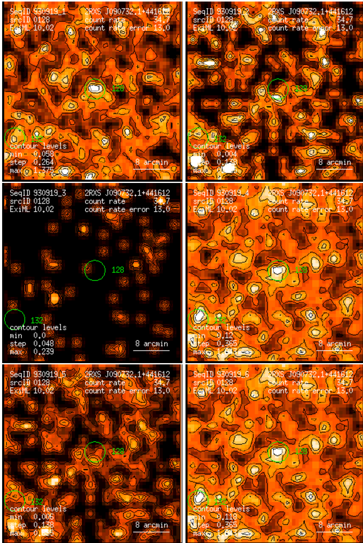
Figure 128: RASS 930919: detection 0128: band rate images, Gaussian filter: (1) PSPC channels 11 – 41, (2) 52 – 90, (3) 91 – 201, (4) 11 – 235, (5) 52 – 201, (6) 11 – 201. Broad band rates in counts/ks. Band rate contour levels in counts/ks/arcmin 2 .
