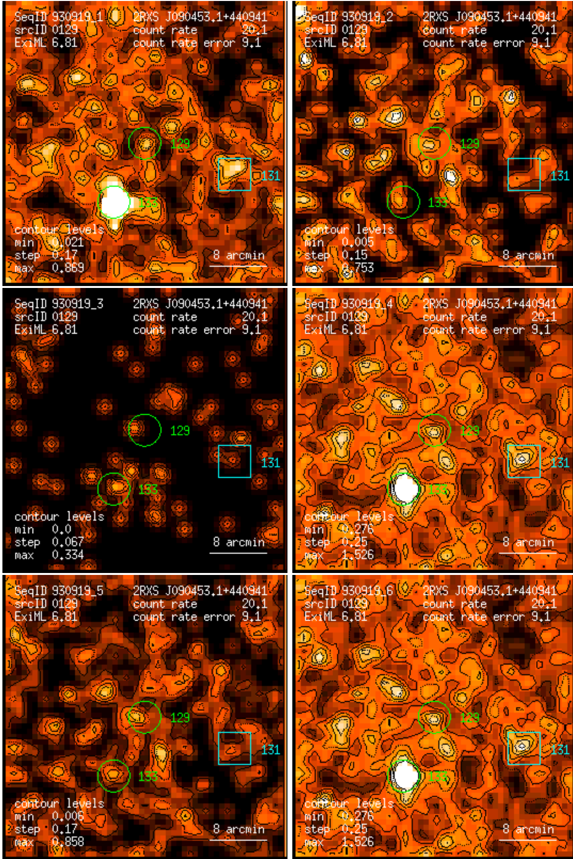
Figure 129: RASS 930919: detection 0129: band rate images, Gaussian filter: (1) PSPC channels 11 – 41, (2) 52 – 90, (3) 91 – 201, (4) 11 – 235, (5) 52 – 201, (6) 11 – 201. Broad band rates in counts/ks. Band rate contour levels in counts/ks/arcmin 2 .
