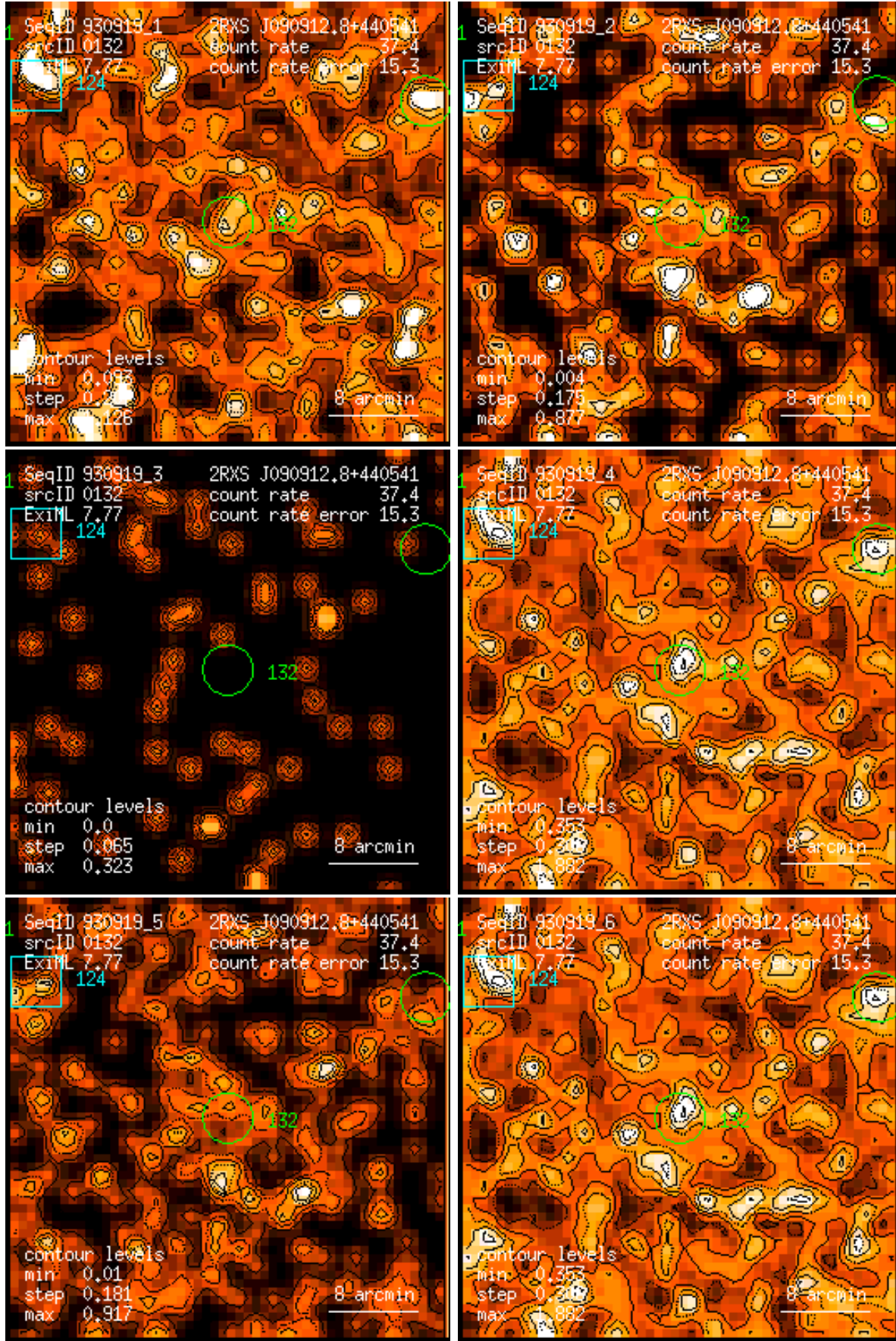
Figure 132: RASS 930919: detection 0132: band rate images, Gaussian filter: (1) PSPC channels 11 – 41, (2) 52 – 90, (3) 91 – 201, (4) 11 – 235, (5) 52 – 201, (6) 11 – 201. Broad band rates in counts/ks. Band rate contour levels in counts/ks/arcmin 2 .
