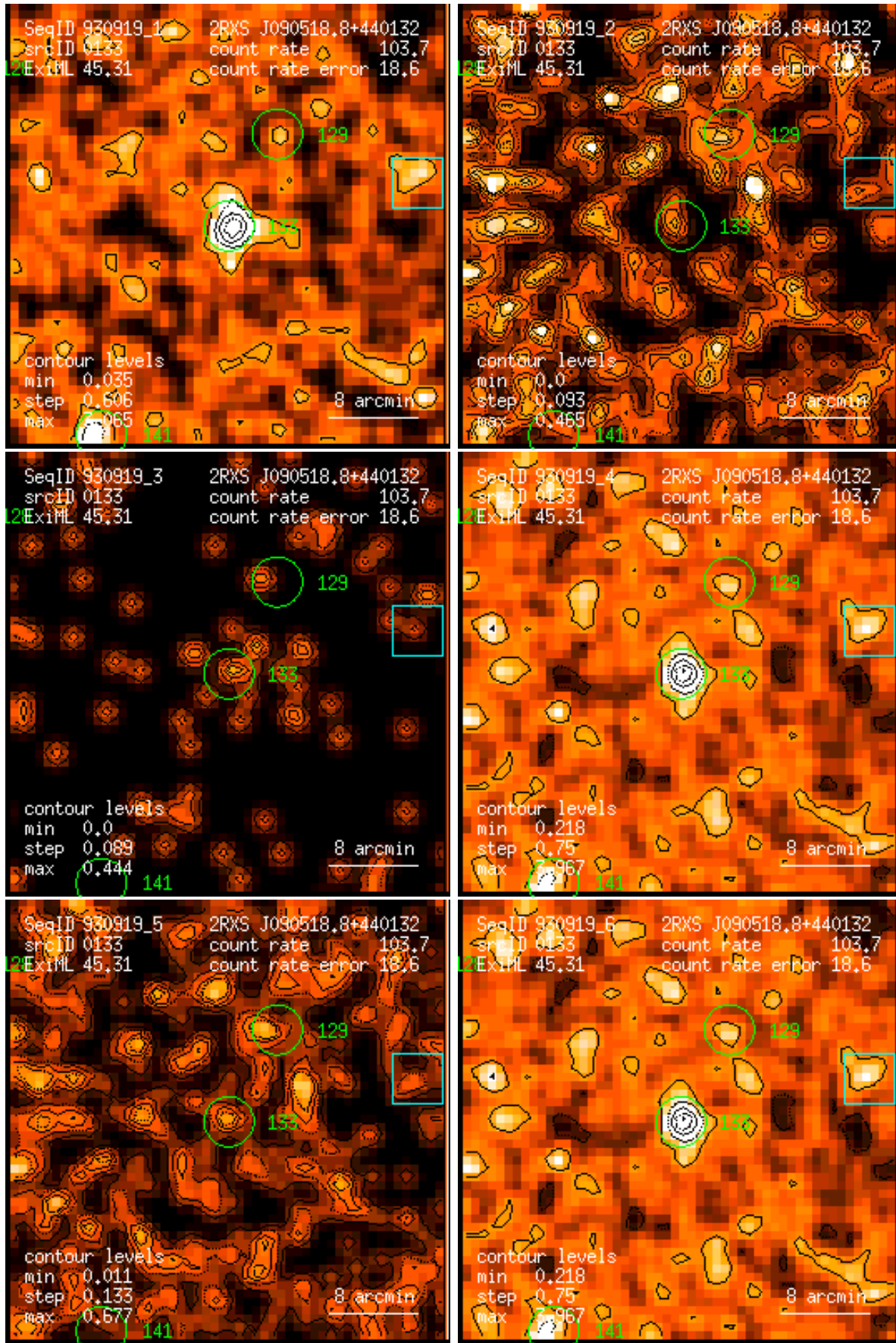
Figure 133: RASS 930919: detection 0133: band rate images, Gaussian filter: (1) PSPC channels 11 – 41, (2) 52 – 90, (3) 91 – 201, (4) 11 – 235, (5) 52 – 201, (6) 11 – 201. Broad band rates in counts/ks. Band rate contour levels in counts/ks/arcmin 2 .
