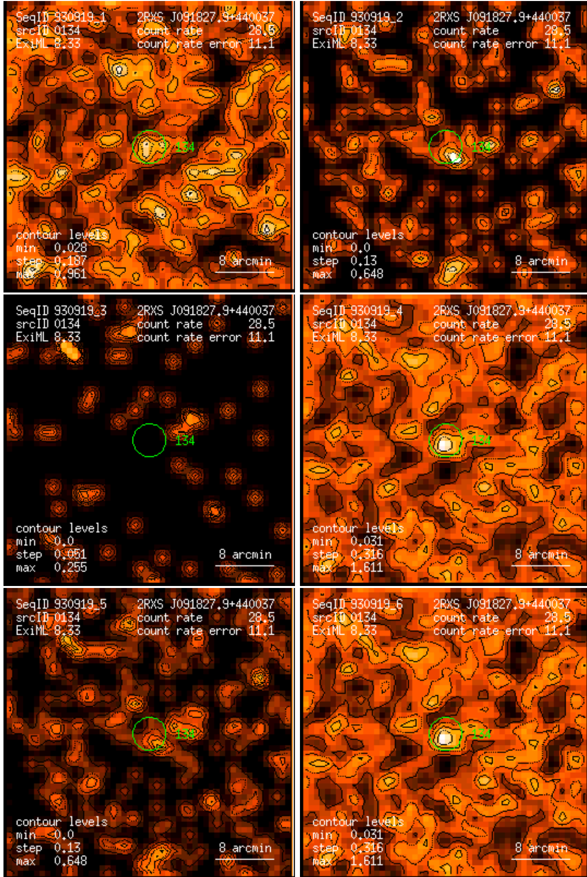
Figure 134: RASS 930919: detection 0134: band rate images, Gaussian filter: (1) PSPC channels 11 – 41, (2) 52 – 90, (3) 91 – 201, (4) 11 – 235, (5) 52 – 201, (6) 11 – 201. Broad band rates in counts/ks. Band rate contour levels in counts/ks/arcmin 2 .
