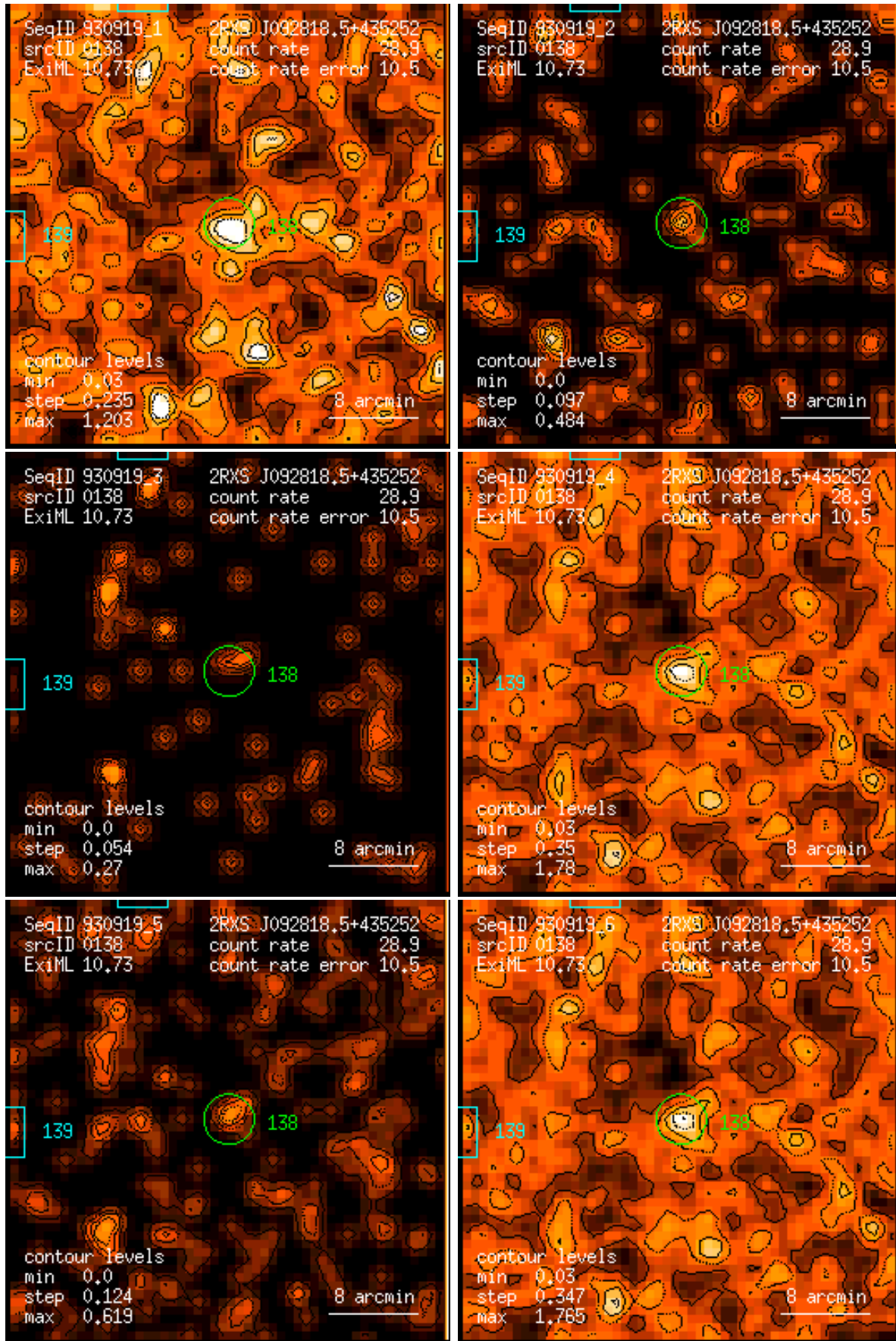
Figure 138: RASS 930919: detection 0138: band rate images, Gaussian filter: (1) PSPC channels 11 – 41, (2) 52 – 90, (3) 91 – 201, (4) 11 – 235, (5) 52 – 201, (6) 11 – 201. Broad band rates in counts/ks. Band rate contour levels in counts/ks/arcmin 2 .
