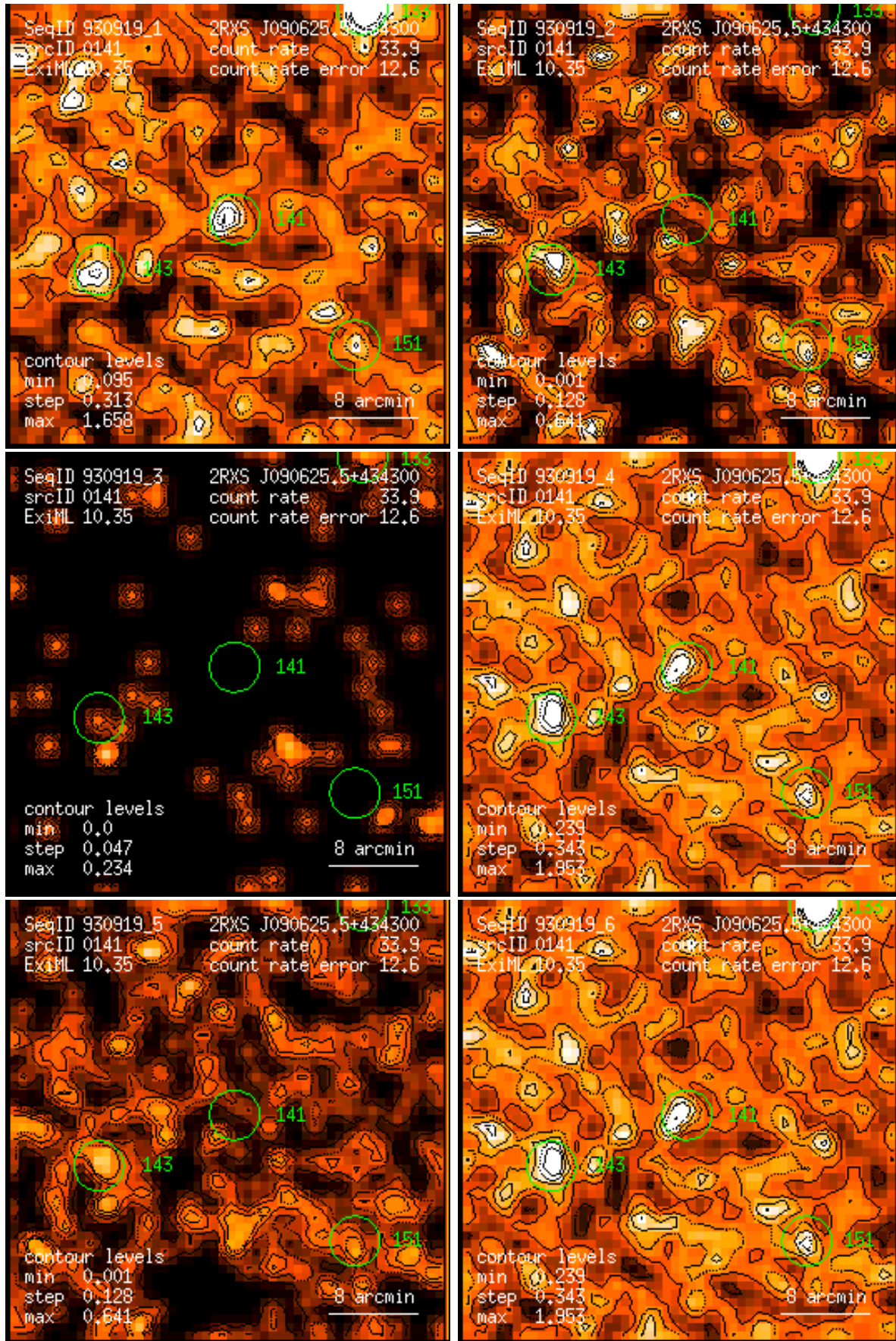
Figure 141: RASS 930919: detection 0141: band rate images, Gaussian filter: (1) PSPC channels 11 – 41, (2) 52 – 90, (3) 91 – 201, (4) 11 – 235, (5) 52 – 201, (6) 11 – 201. Broad band rates in counts/ks. Band rate contour levels in counts/ks/arcmin 2 .
