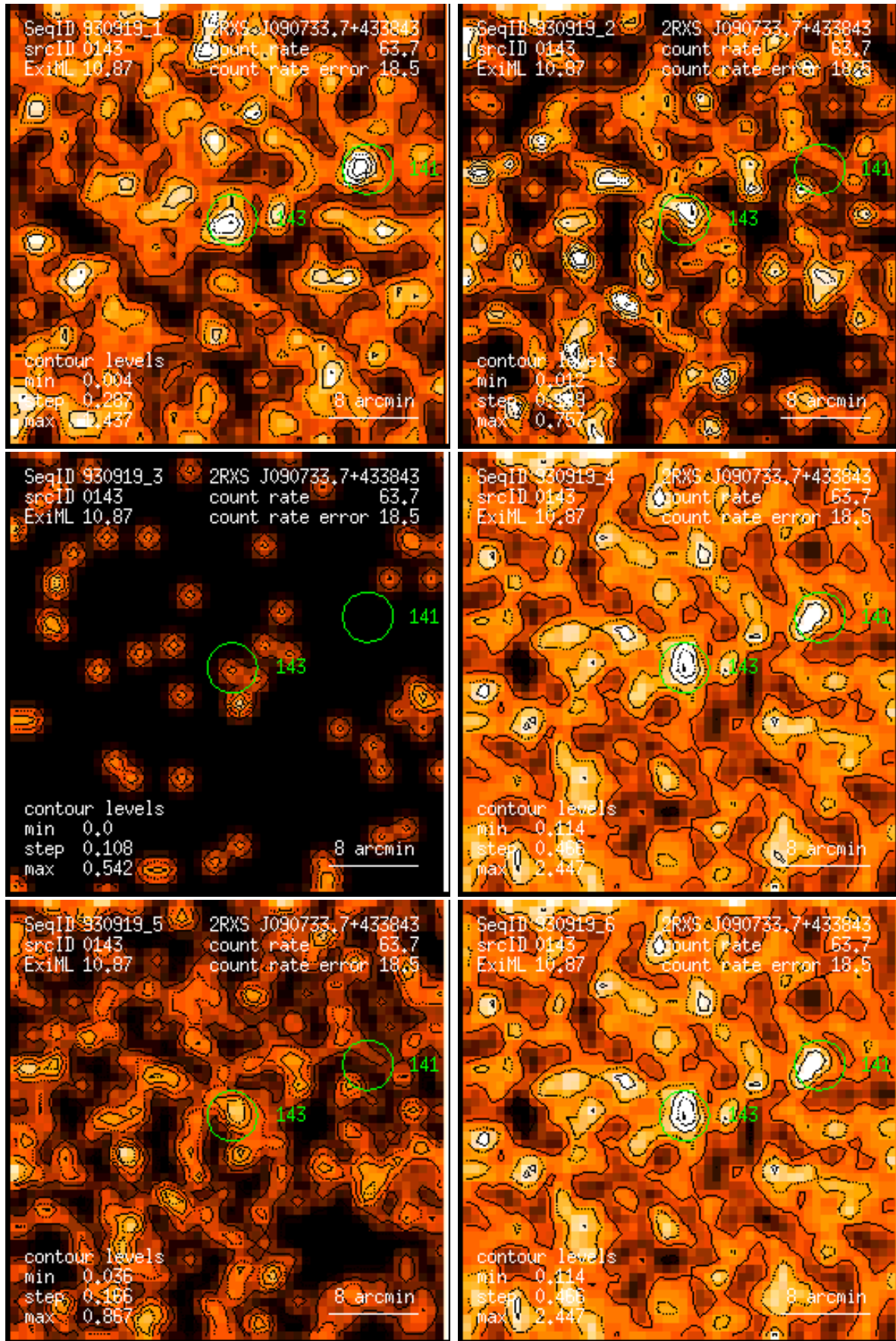
Figure 143: RASS 930919: detection 0143: band rate images, Gaussian filter: (1) PSPC channels 11 – 41, (2) 52 – 90, (3) 91 – 201, (4) 11 – 235, (5) 52 – 201, (6) 11 – 201. Broad band rates in counts/ks. Band rate contour levels in counts/ks/arcmin 2 .
