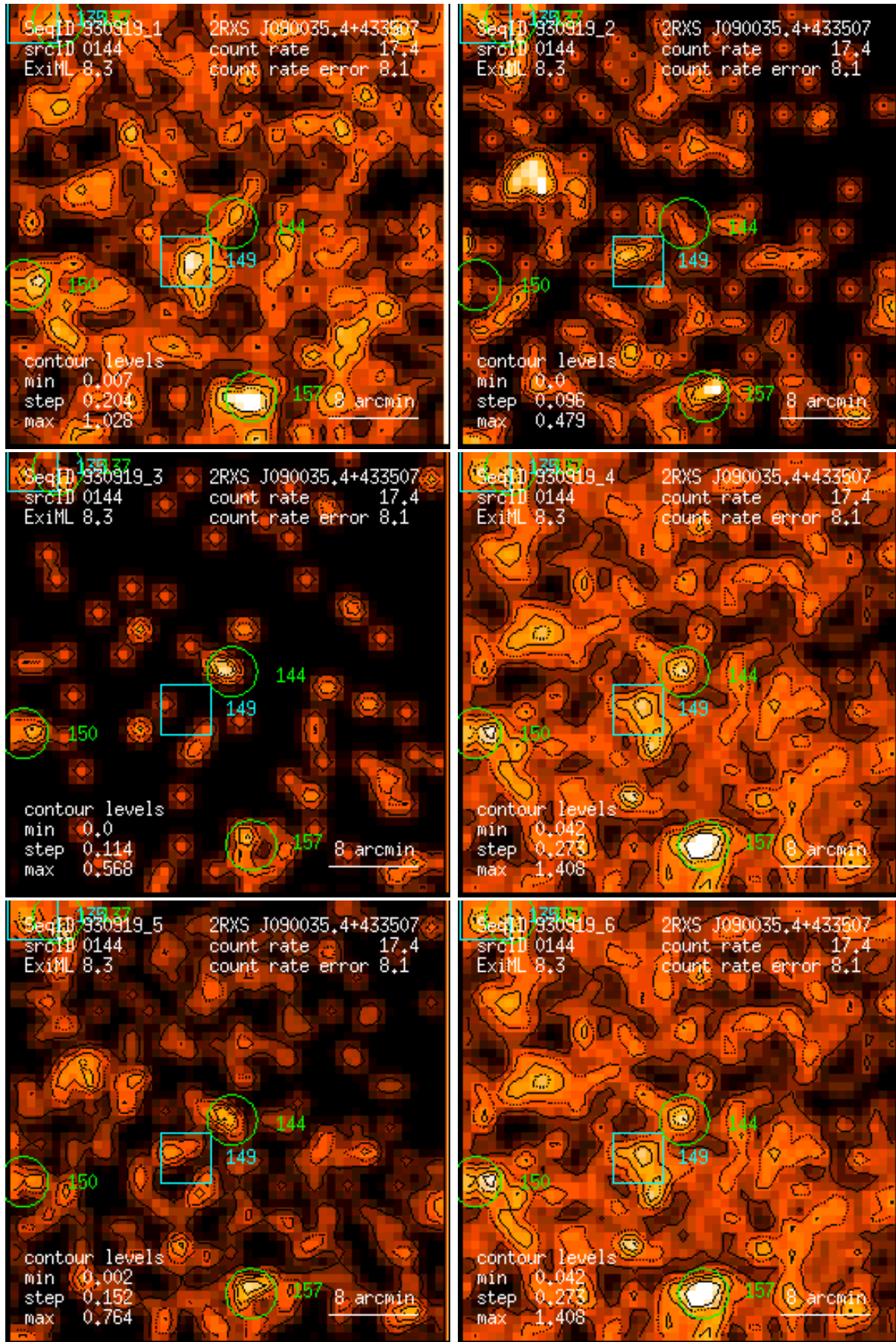
Figure 144: RASS 930919: detection 0144: band rate images, Gaussian filter: (1) PSPC channels 11 – 41, (2) 52 – 90, (3) 91 – 201, (4) 11 – 235, (5) 52 – 201, (6) 11 – 201. Broad band rates in counts/ks. Band rate contour levels in counts/ks/arcmin 2 .
