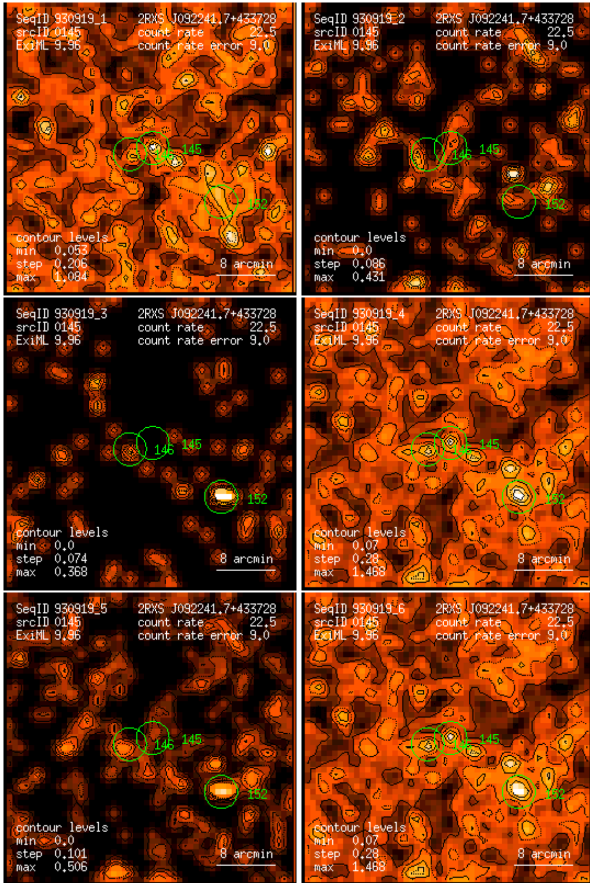
Figure 145: RASS 930919: detection 0145: band rate images, Gaussian filter: (1) PSPC channels 11 – 41, (2) 52 – 90, (3) 91 – 201, (4) 11 – 235, (5) 52 – 201, (6) 11 – 201. Broad band rates in counts/ks. Band rate contour levels in counts/ks/arcmin 2 .
