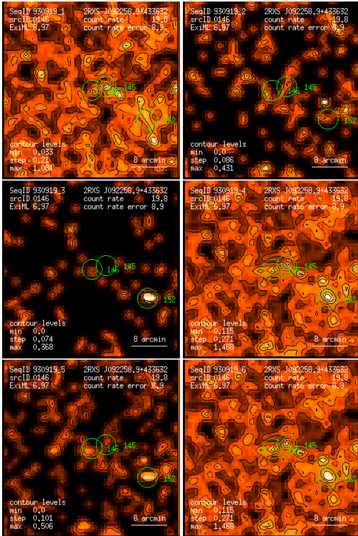
Figure 146: RASS 930919: detection 0146: band rate images, Gaussian filter: (1) PSPC channels 11 – 41, (2) 52 – 90, (3) 91 – 201, (4) 11 – 235, (5) 52 – 201, (6) 11 – 201. Broad band rates in counts/ks. Band rate contour levels in counts/ks/arcmin 2 .
