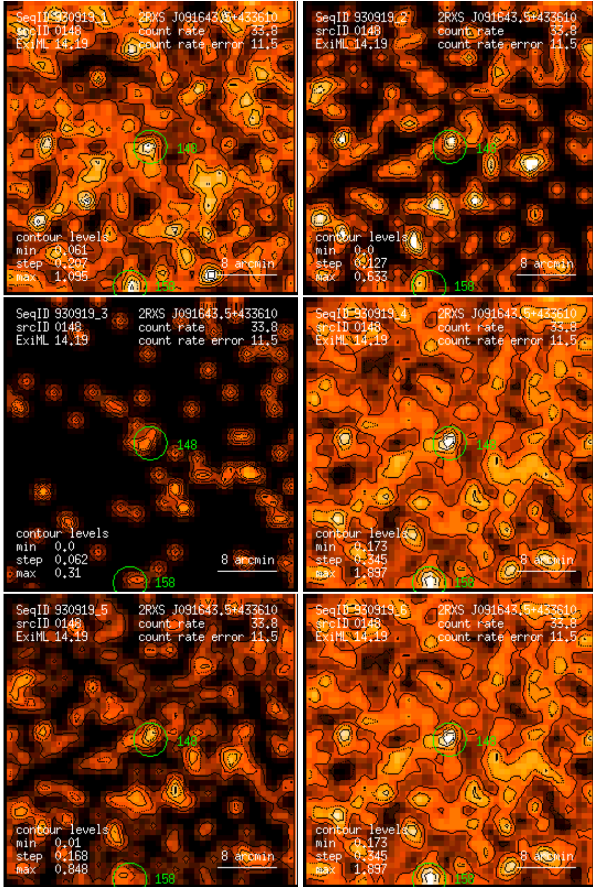
Figure 148: RASS 930919: detection 0148: band rate images, Gaussian filter: (1) PSPC channels 11 – 41, (2) 52 – 90, (3) 91 – 201, (4) 11 – 235, (5) 52 – 201, (6) 11 – 201. Broad band rates in counts/ks. Band rate contour levels in counts/ks/arcmin 2 .
