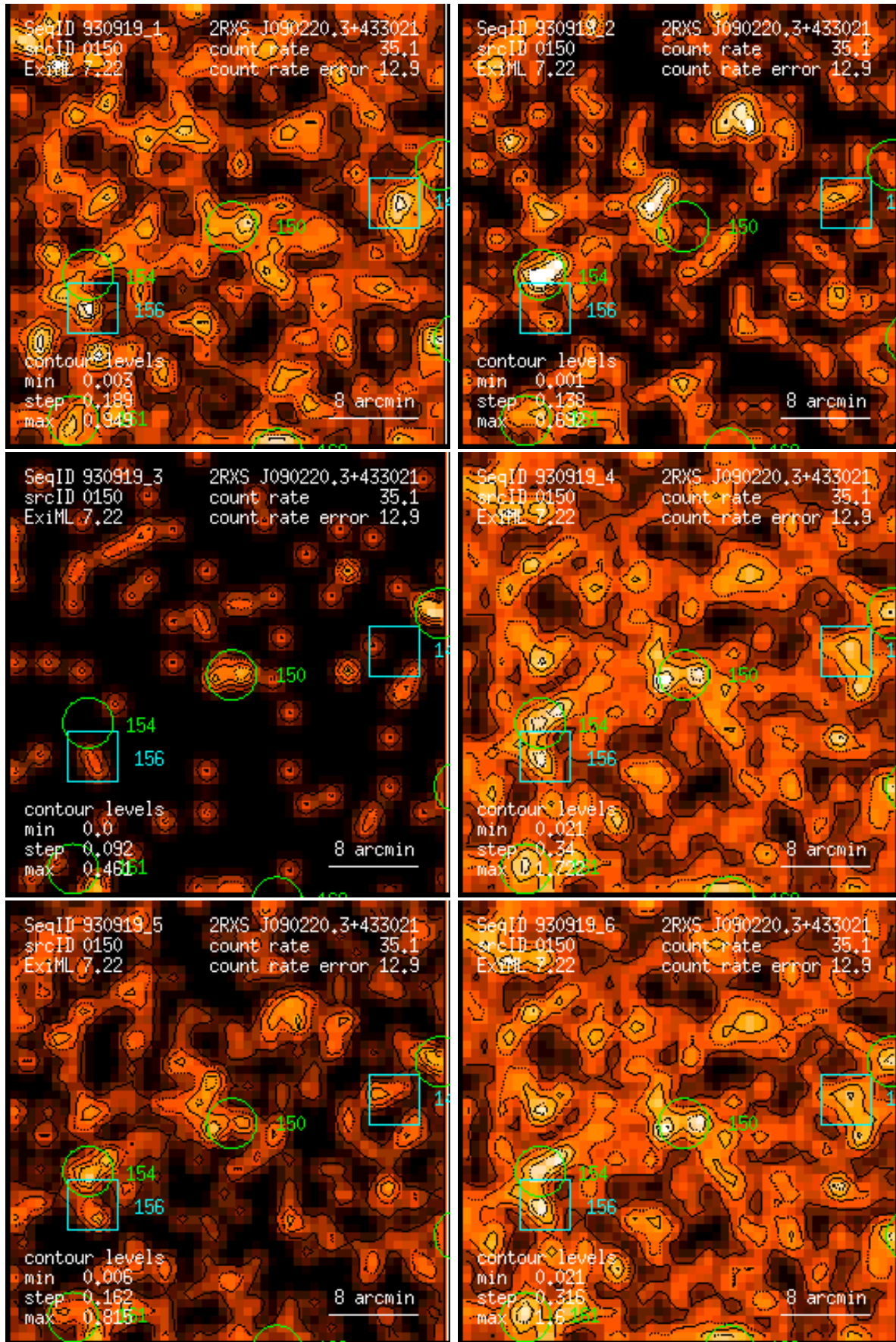
Figure 150: RASS 930919: detection 0150: band rate images, Gaussian filter: (1) PSPC channels 11 – 41, (2) 52 – 90, (3) 91 – 201, (4) 11 – 235, (5) 52 – 201, (6) 11 – 201. Broad band rates in counts/ks. Band rate contour levels in counts/ks/arcmin 2 .
