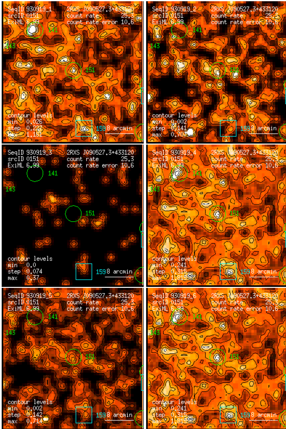
Figure 151: RASS 930919: detection 0151: band rate images, Gaussian filter: (1) PSPC channels 11 – 41, (2) 52 – 90, (3) 91 – 201, (4) 11 – 235, (5) 52 – 201, (6) 11 – 201. Broad band rates in counts/ks. Band rate contour levels in counts/ks/arcmin 2 .
