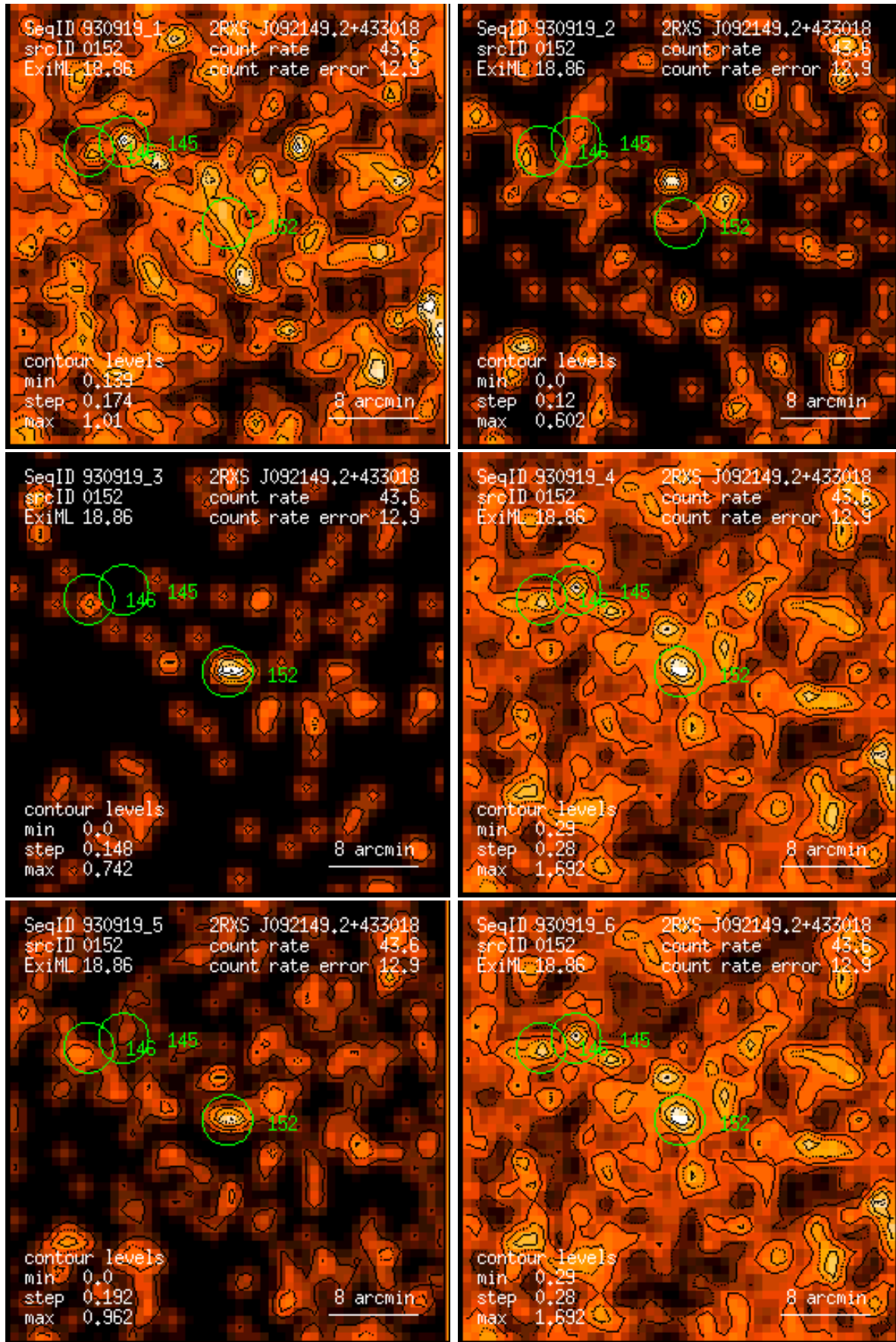
Figure 152: RASS 930919: detection 0152: band rate images, Gaussian filter: (1) PSPC channels 11 – 41, (2) 52 – 90, (3) 91 – 201, (4) 11 – 235, (5) 52 – 201, (6) 11 – 201. Broad band rates in counts/ks. Band rate contour levels in counts/ks/arcmin 2 .
