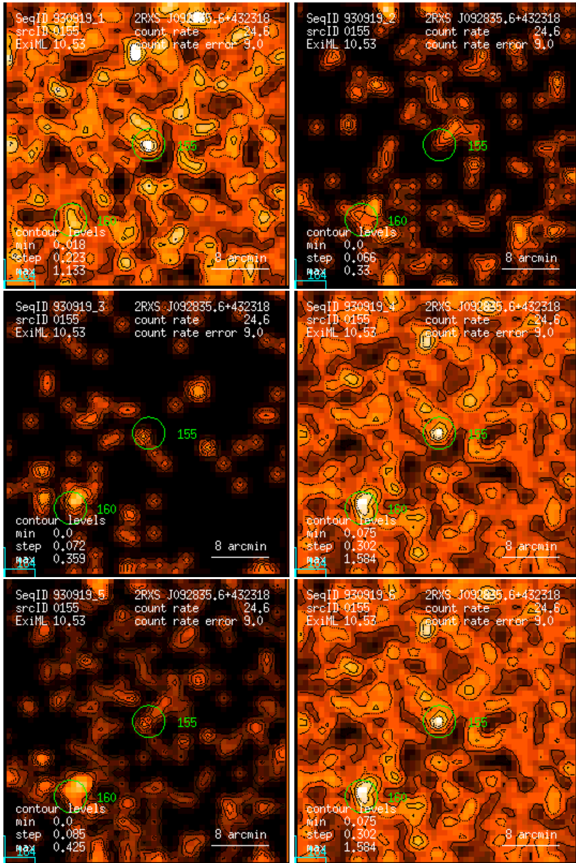
Figure 155: RASS 930919: detection 0155: band rate images, Gaussian filter: (1) PSPC channels 11 – 41, (2) 52 – 90, (3) 91 – 201, (4) 11 – 235, (5) 52 – 201, (6) 11 – 201. Broad band rates in counts/ks. Band rate contour levels in counts/ks/arcmin 2 .
