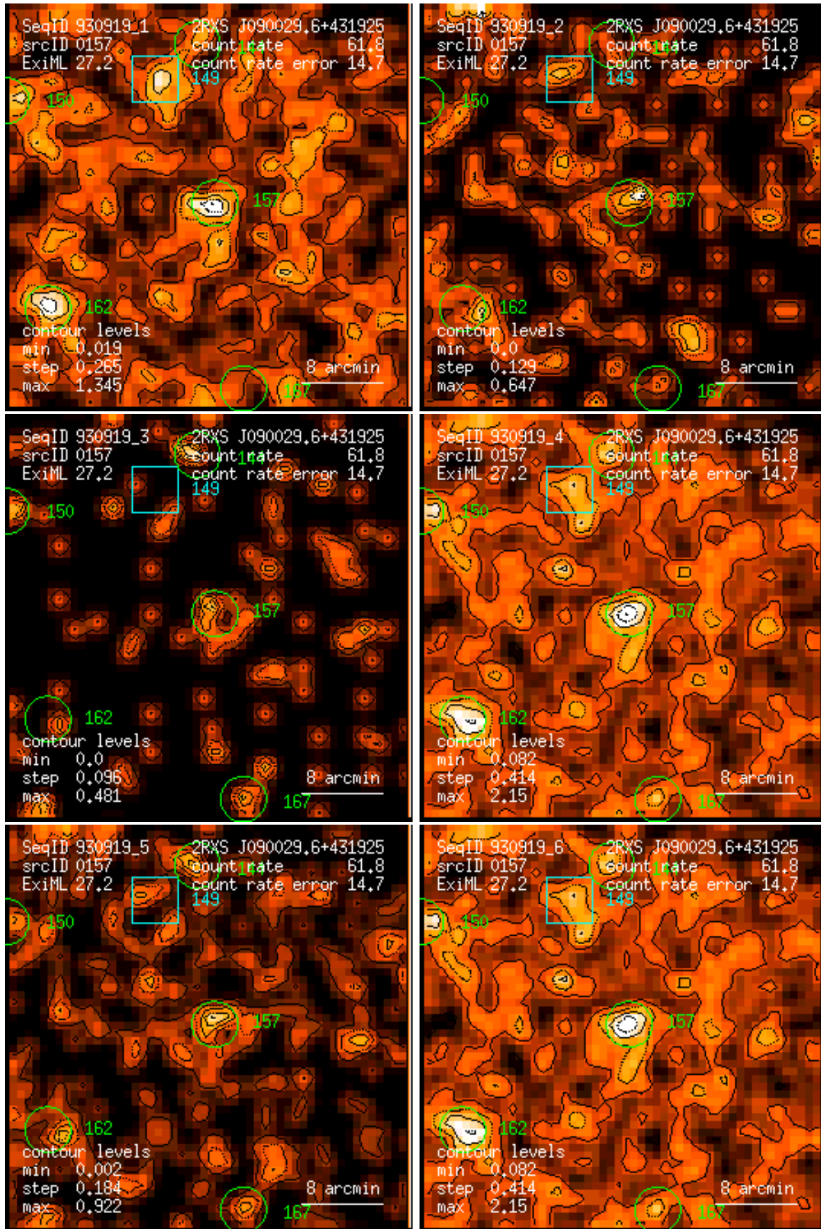
Figure 157: RASS 930919: detection 0157: band rate images, Gaussian filter: (1) PSPC channels 11 – 41, (2) 52 – 90, (3) 91 – 201, (4) 11 – 235, (5) 52 – 201, (6) 11 – 201. Broad band rates in counts/ks. Band rate contour levels in counts/ks/arcmin 2 .
