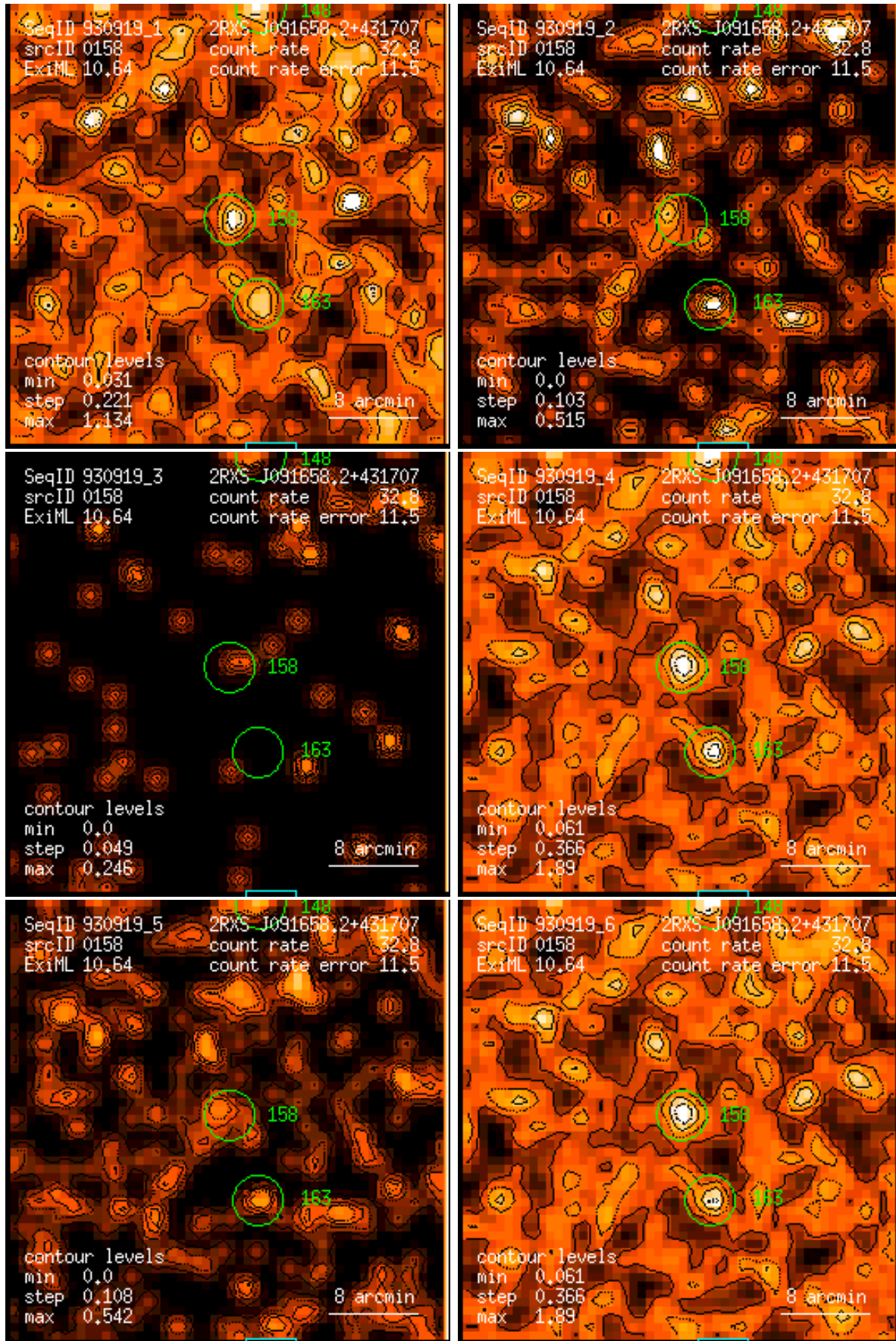
Figure 158: RASS 930919: detection 0158: band rate images, Gaussian filter: (1) PSPC channels 11 – 41, (2) 52 – 90, (3) 91 – 201, (4) 11 – 235, (5) 52 – 201, (6) 11 – 201. Broad band rates in counts/ks. Band rate contour levels in counts/ks/arcmin 2 .
