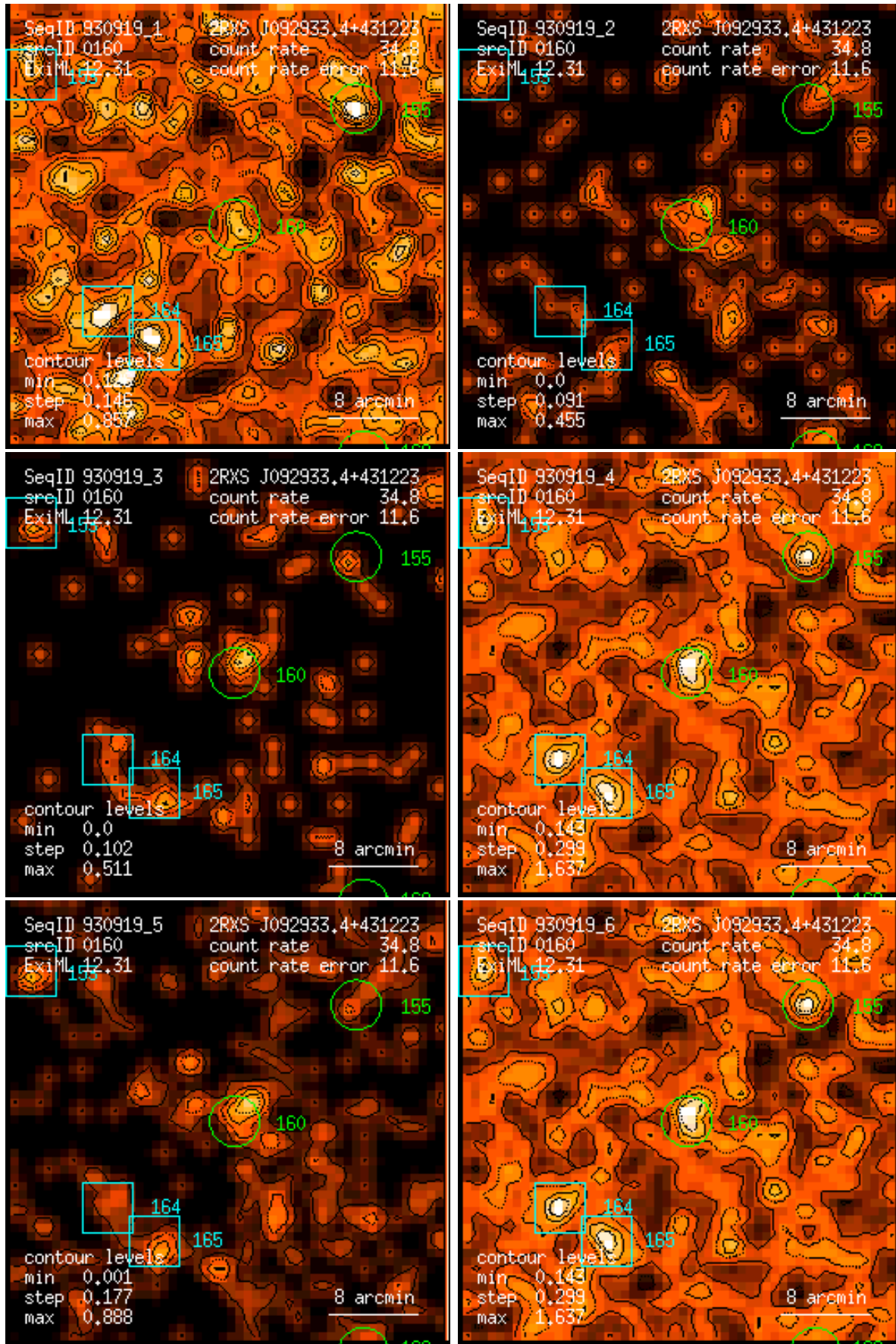
Figure 160: RASS 930919: detection 0160: band rate images, Gaussian filter: (1) PSPC channels 11 – 41, (2) 52 – 90, (3) 91 – 201, (4) 11 – 235, (5) 52 – 201, (6) 11 – 201. Broad band rates in counts/ks. Band rate contour levels in counts/ks/arcmin 2 .
