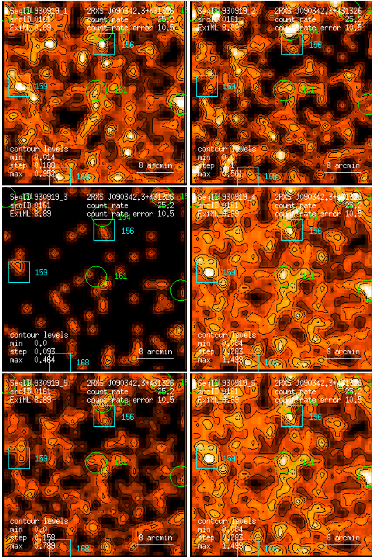
Figure 161: RASS 930919: detection 0161: band rate images, Gaussian filter: (1) PSPC channels 11 – 41, (2) 52 – 90, (3) 91 – 201, (4) 11 – 235, (5) 52 – 201, (6) 11 – 201. Broad band rates in counts/ks. Band rate contour levels in counts/ks/arcmin 2 .
