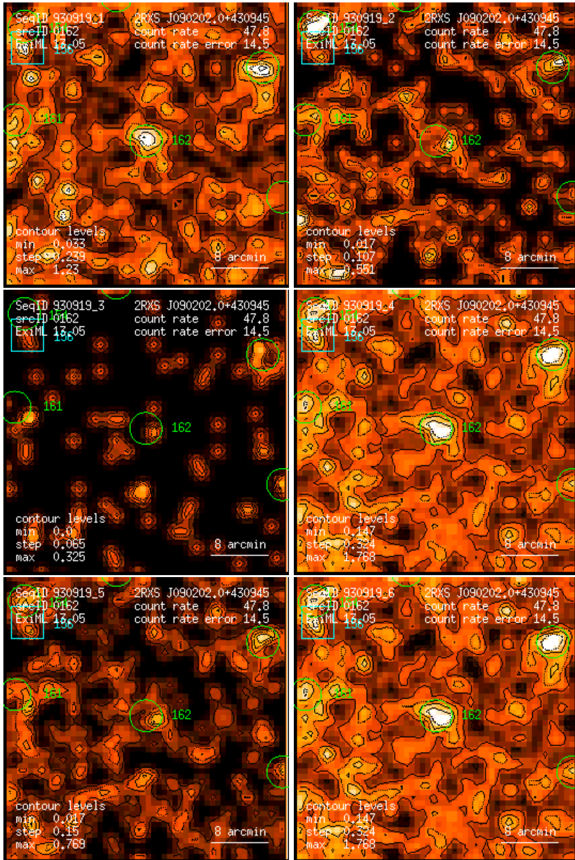
Figure 162: RASS 930919: detection 0162: band rate images, Gaussian filter: (1) PSPC channels 11 – 41, (2) 52 – 90, (3) 91 – 201, (4) 11 – 235, (5) 52 – 201, (6) 11 – 201. Broad band rates in counts/ks. Band rate contour levels in counts/ks/arcmin 2 .
