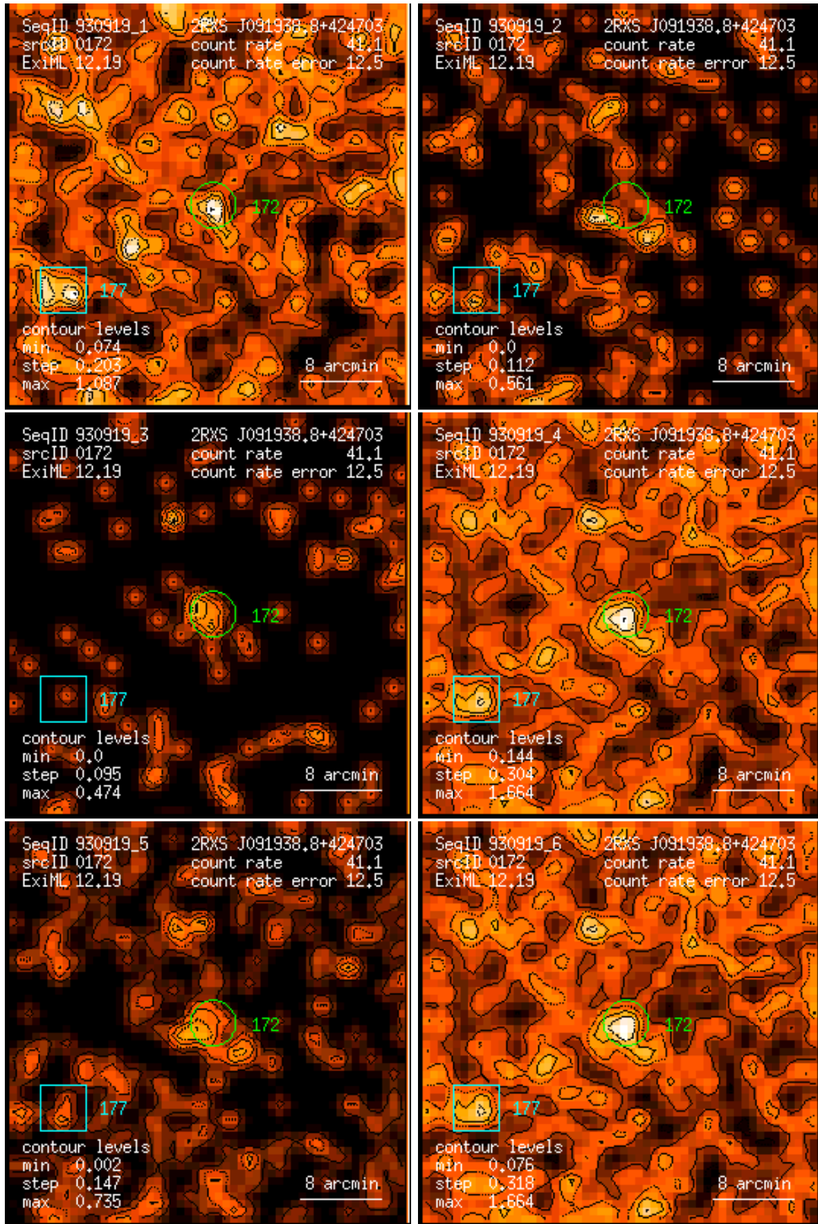
Figure 172: RASS 930919: detection 0172: band rate images, Gaussian filter: (1) PSPC channels 11 – 41, (2) 52 – 90, (3) 91 – 201, (4) 11 – 235, (5) 52 – 201, (6) 11 – 201. Broad band rates in counts/ks. Band rate contour levels in counts/ks/arcmin 2 .
