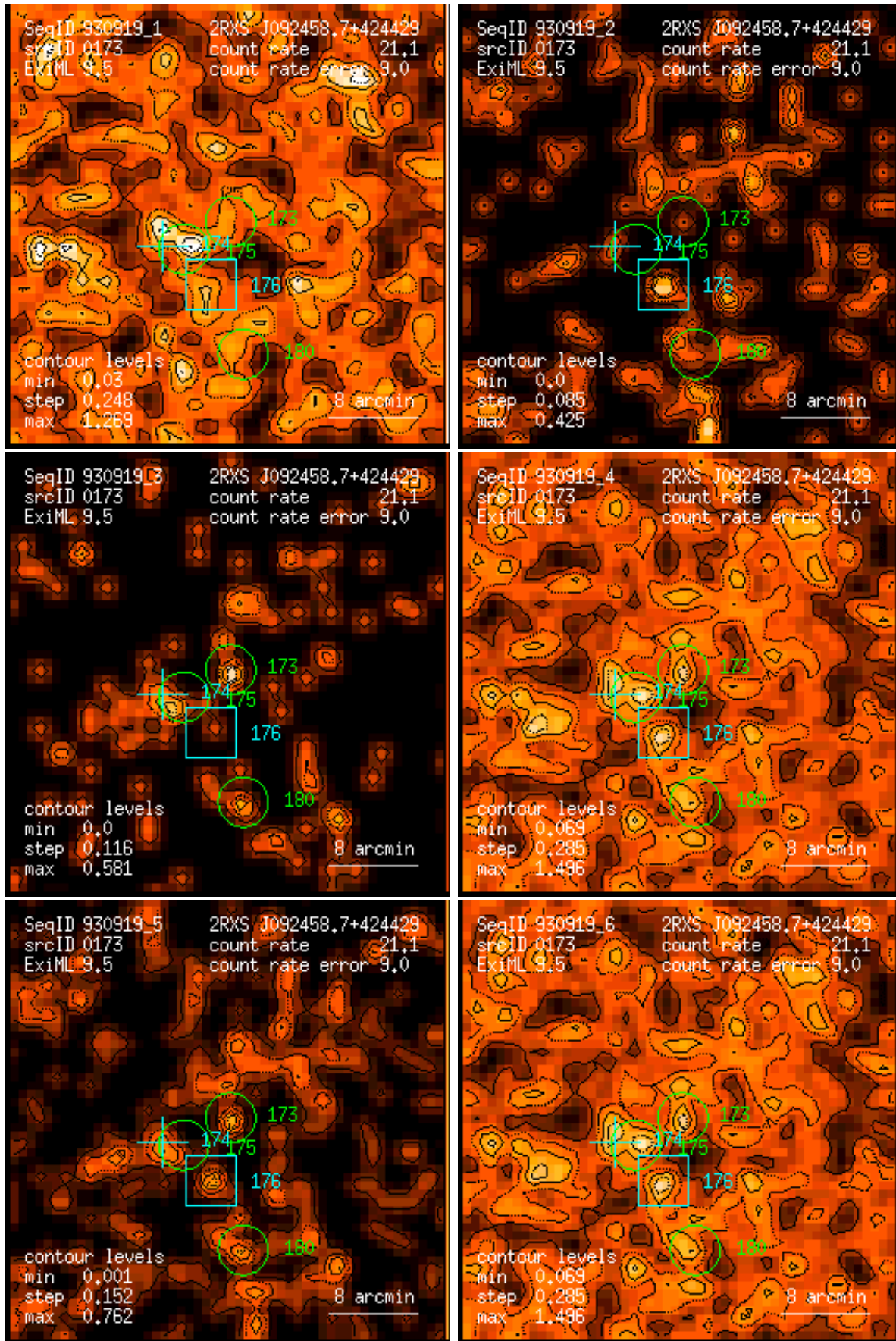
Figure 173: RASS 930919: detection 0173: band rate images, Gaussian filter: (1) PSPC channels 11 – 41, (2) 52 – 90, (3) 91 – 201, (4) 11 – 235, (5) 52 – 201, (6) 11 – 201. Broad band rates in counts/ks. Band rate contour levels in counts/ks/arcmin 2 .
