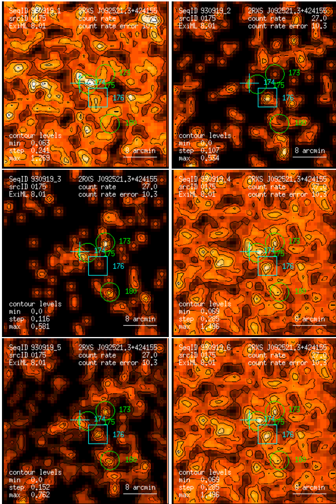
Figure 175: RASS 930919: detection 0175: band rate images, Gaussian filter: (1) PSPC channels 11 – 41, (2) 52 – 90, (3) 91 – 201, (4) 11 – 235, (5) 52 – 201, (6) 11 – 201. Broad band rates in counts/ks. Band rate contour levels in counts/ks/arcmin 2 .
