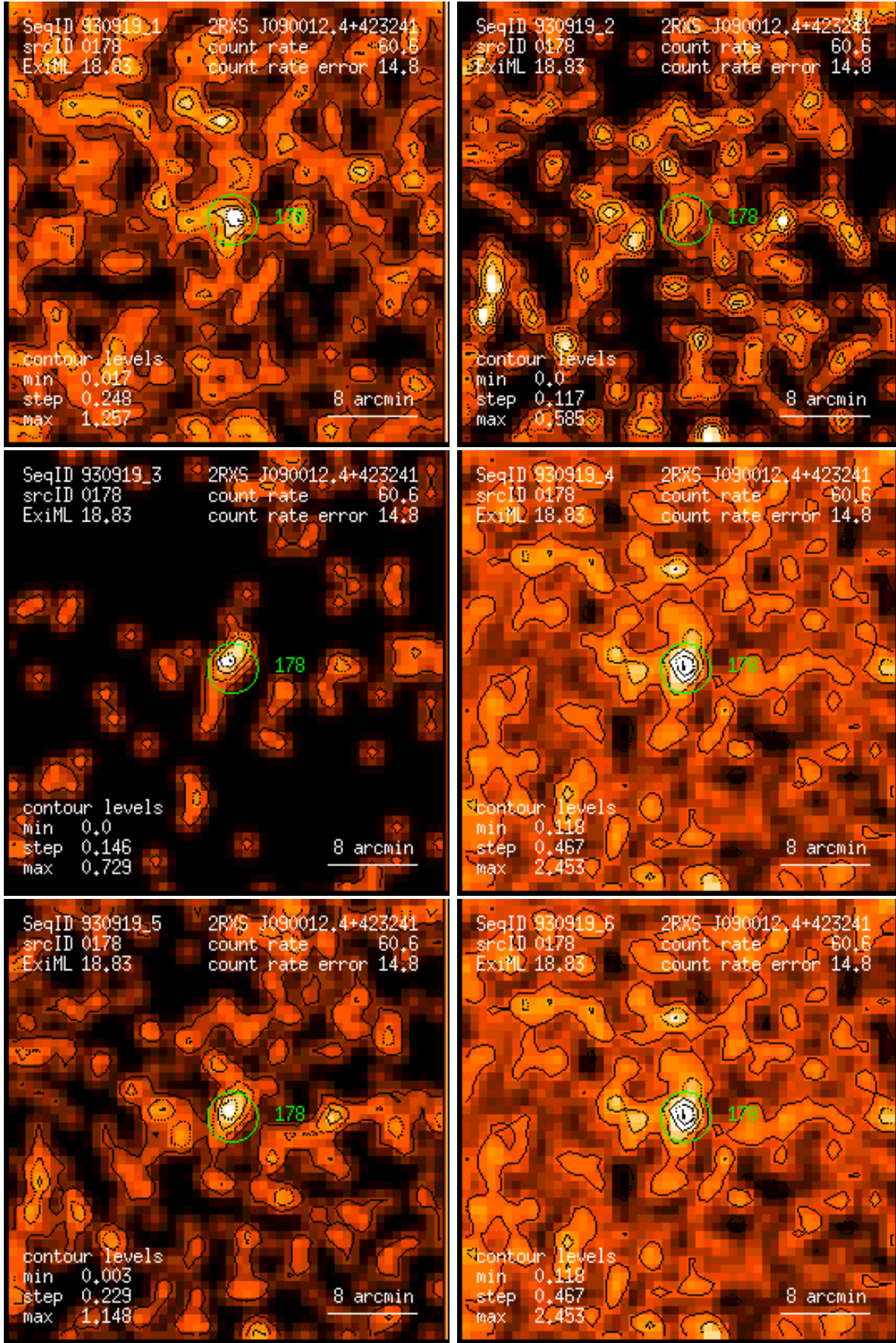
Figure 178: RASS 930919: detection 0178: band rate images, Gaussian filter: (1) PSPC channels 11 – 41, (2) 52 – 90, (3) 91 – 201, (4) 11 – 235, (5) 52 – 201, (6) 11 – 201. Broad band rates in counts/ks. Band rate contour levels in counts/ks/arcmin 2 .
