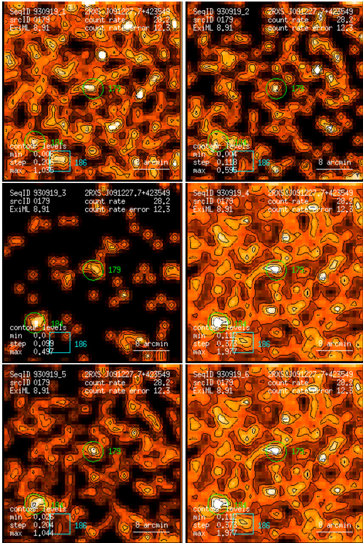
Figure 179: RASS 930919: detection 0179: band rate images, Gaussian filter: (1) PSPC channels 11 – 41, (2) 52 – 90, (3) 91 – 201, (4) 11 – 235, (5) 52 – 201, (6) 11 – 201. Broad band rates in counts/ks. Band rate contour levels in counts/ks/arcmin 2 .
