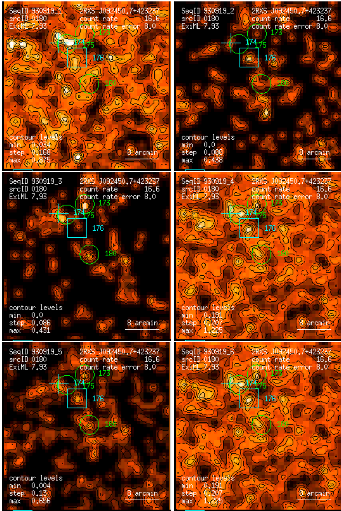
Figure 180: RASS 930919: detection 0180: band rate images, Gaussian filter: (1) PSPC channels 11 – 41, (2) 52 – 90, (3) 91 – 201, (4) 11 – 235, (5) 52 – 201, (6) 11 – 201. Broad band rates in counts/ks. Band rate contour levels in counts/ks/arcmin 2 .
