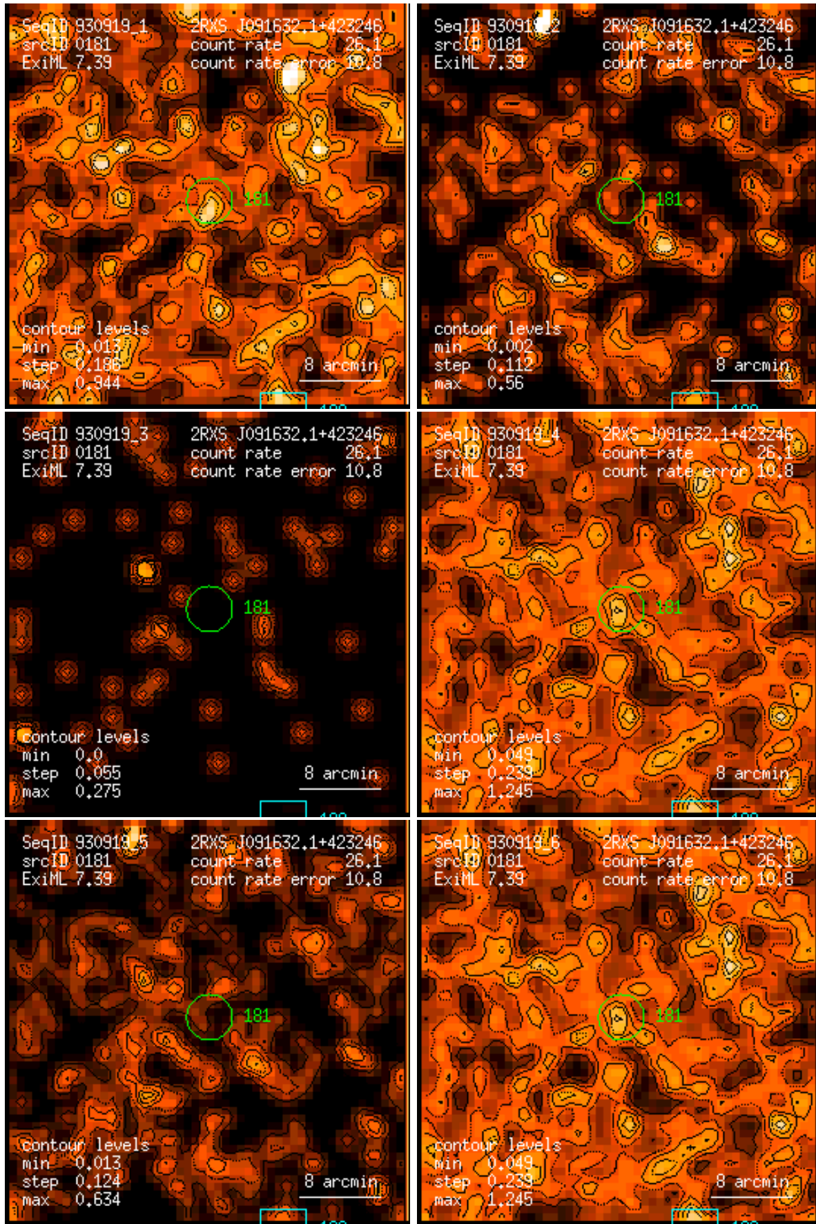
Figure 181: RASS 930919: detection 0181: band rate images, Gaussian filter: (1) PSPC channels 11 – 41, (2) 52 – 90, (3) 91 – 201, (4) 11 – 235, (5) 52 – 201, (6) 11 – 201. Broad band rates in counts/ks. Band rate contour levels in counts/ks/arcmin 2 .
