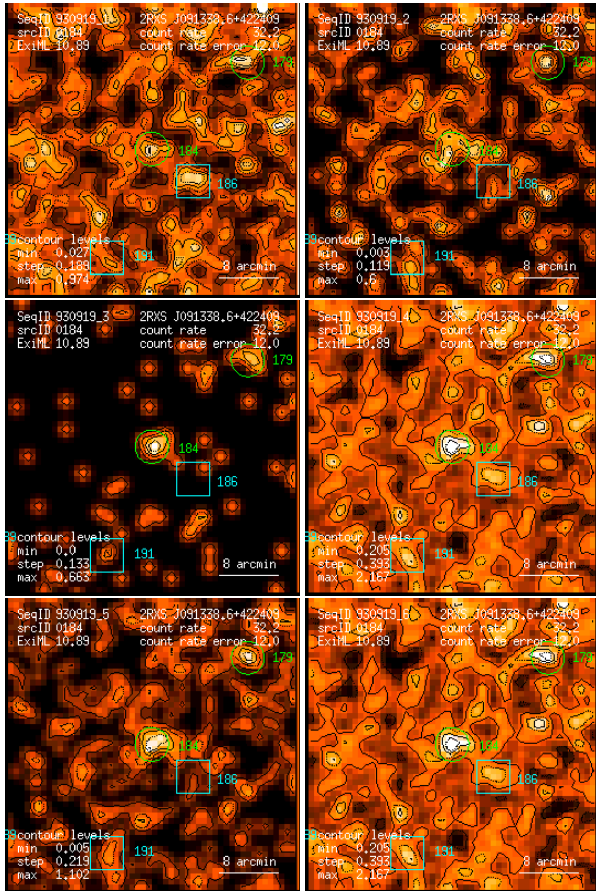
Figure 184: RASS 930919: detection 0184: band rate images, Gaussian filter: (1) PSPC channels 11 – 41, (2) 52 – 90, (3) 91 – 201, (4) 11 – 235, (5) 52 – 201, (6) 11 – 201. Broad band rates in counts/ks. Band rate contour levels in counts/ks/arcmin 2 .
