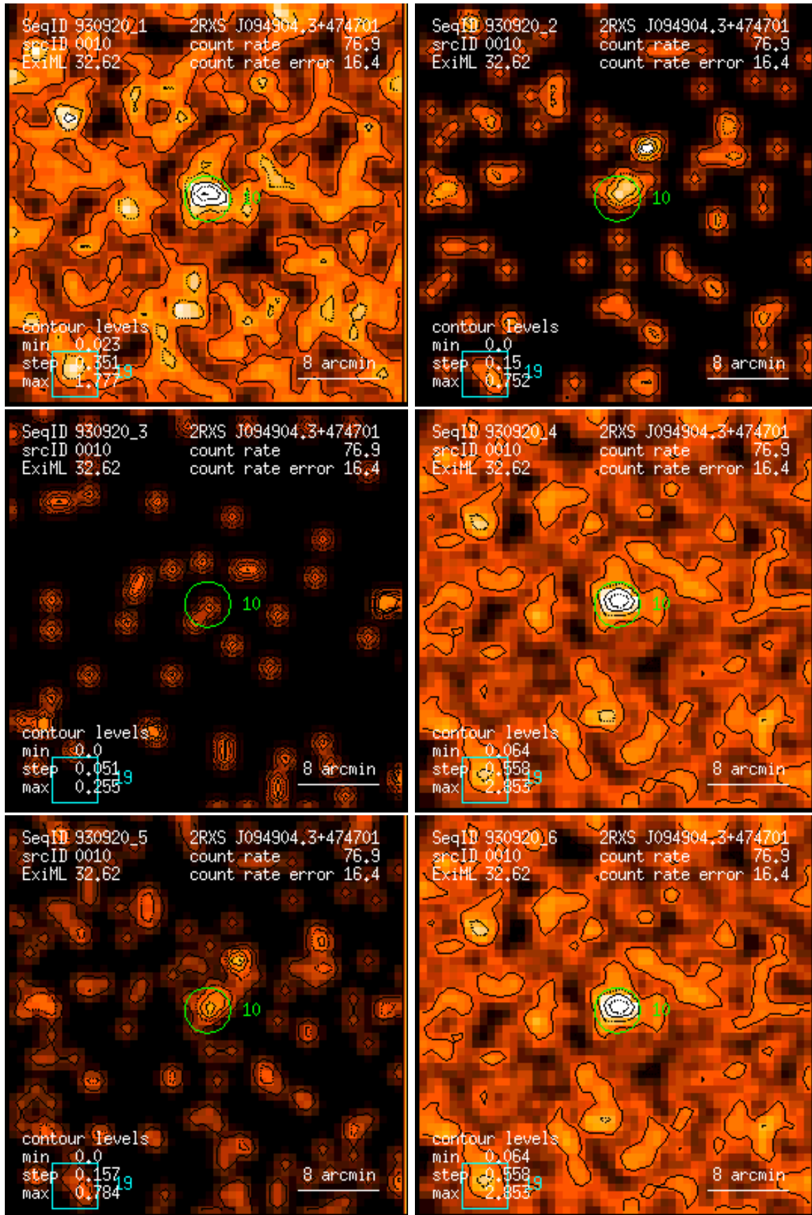
Figure 10: RASS 930920: detection 0010: band rate images, Gaussian filter: (1) PSPC channels 11 – 41, (2) 52 – 90, (3) 91 – 201, (4) 11 – 235, (5) 52 – 201, (6) 11 – 201. Broad band rates in counts/ks. Band rate contour levels in counts/ks/arcmin 2 .
